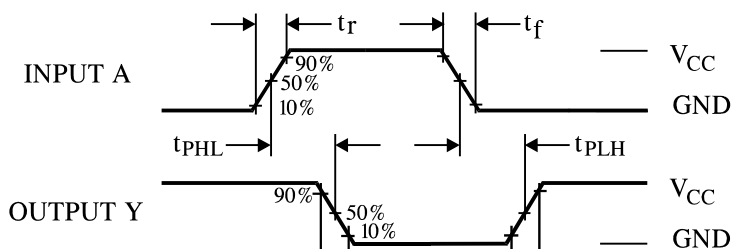
Figure 1. Switching Waveforms
