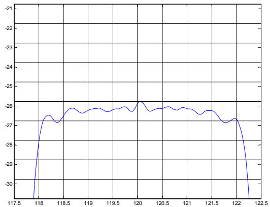
Phase Linearity( f_0 \pm 2\text{MHz} )
