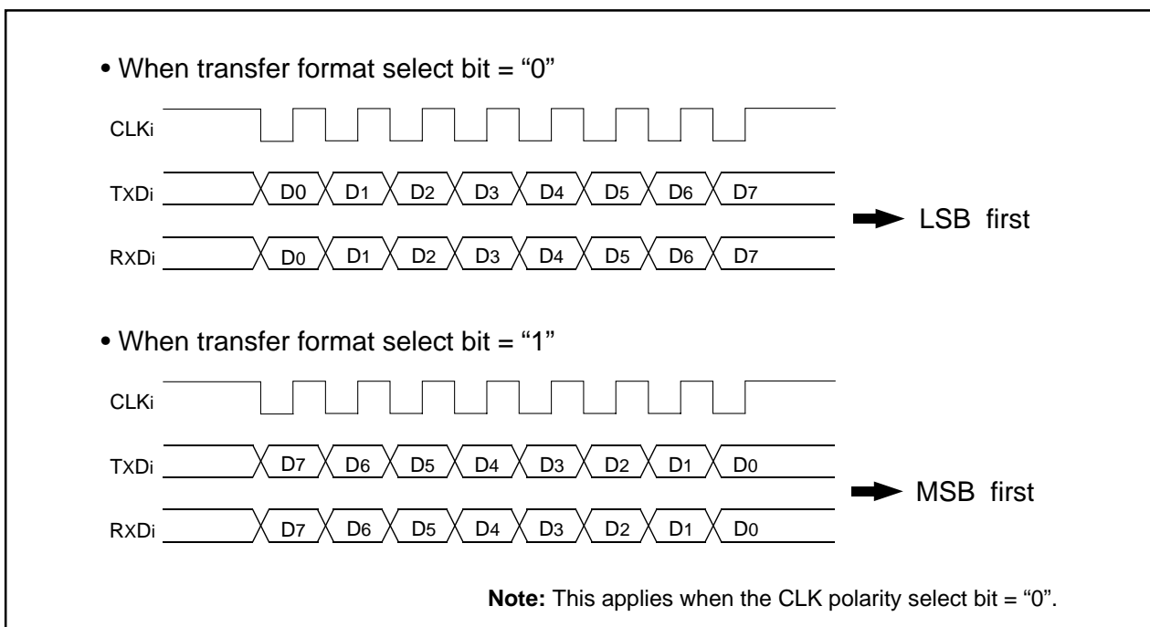
Figure 2.11.18 Transfer format
