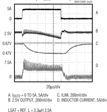
INDUCTOR-SATURATION PROTECTION ( \Delta V_{ILIM} = 200mV )
