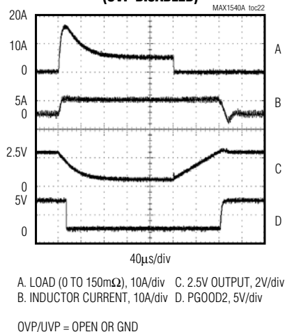
OUTPUT OVERLOAD (UVP DISABLED)
