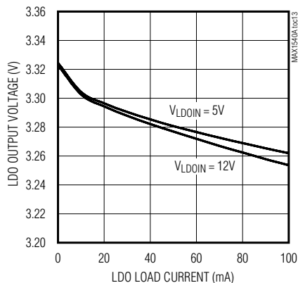
LINEAR-REGULATOR OUTPUT (LD00OUT) vs. LOAD CURRENT
