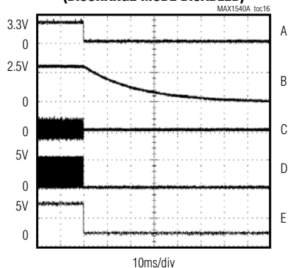
SHUTDOWN WAVEFORM (DISCHARGE MODE DISABLED)
