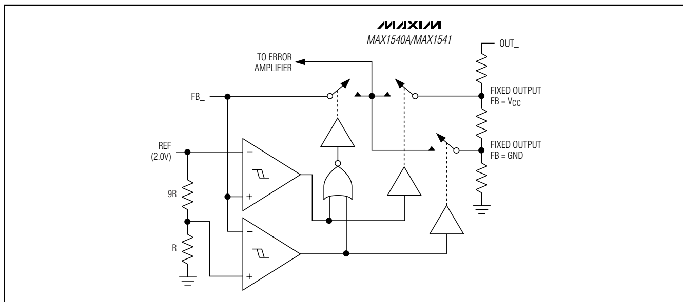
Figure 10. MAX1540A/MAX1541 Dual Mode Feedback Decoder
