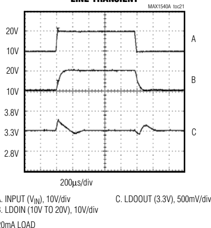
LINEAR-REGULATOR LINE TRANSIENT
