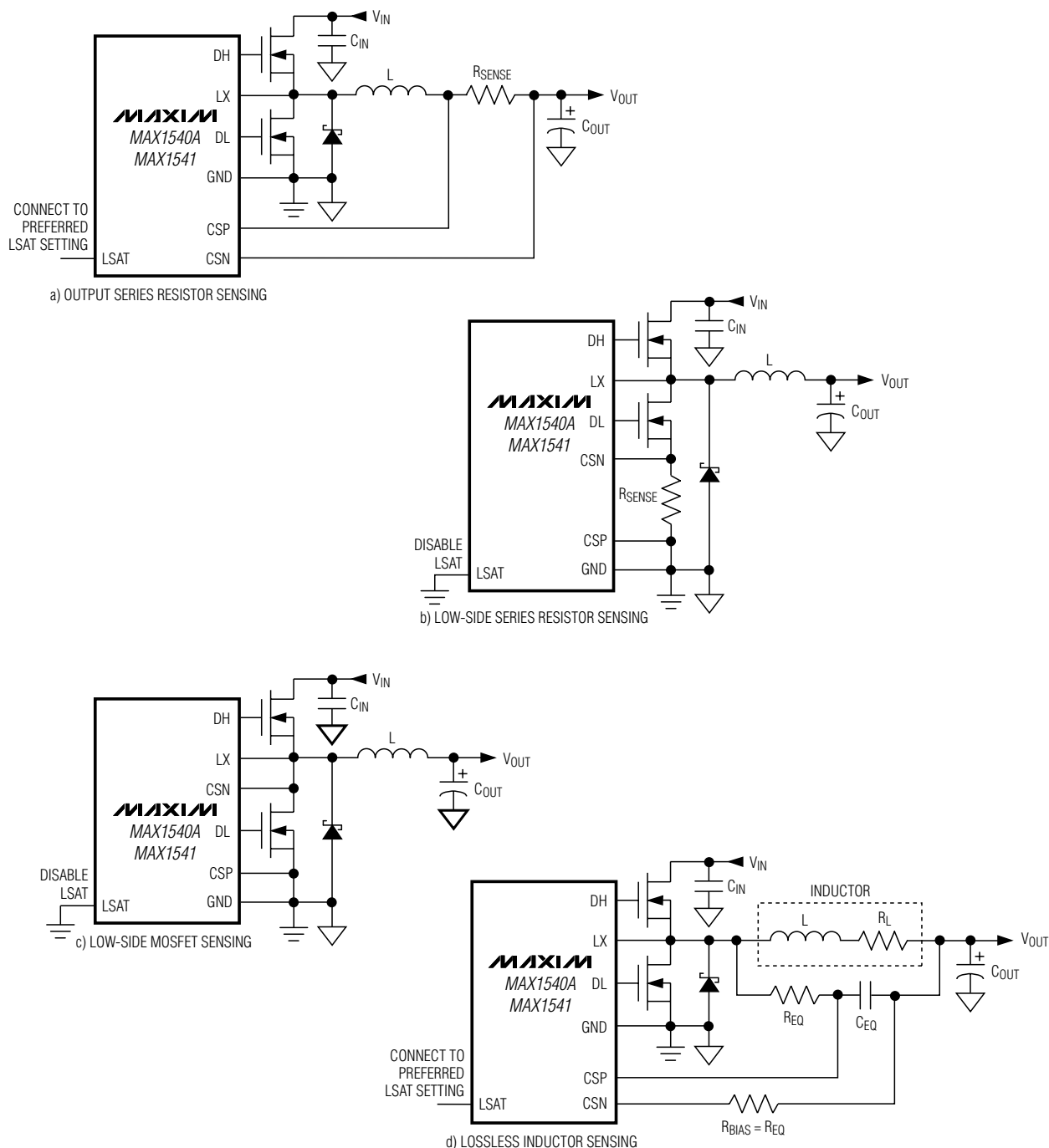
Figure 14. Current-Sense Configurations
