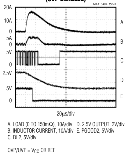
OUTPUT OVERLOAD (UVP ENABLED)
