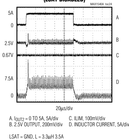
INDUCTOR-SATURATION PROTECTION (LSAT DISABLED)
