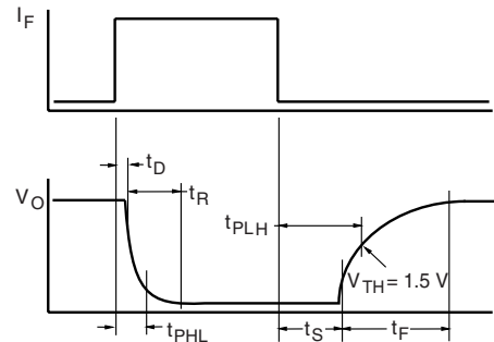
Fig. 2 - Switching Waveform
