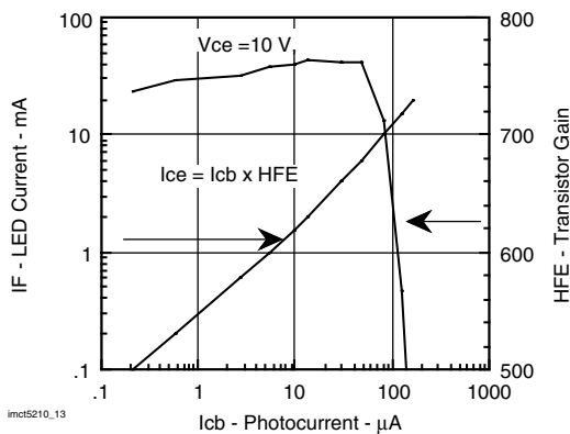
Fig. 13 - Transfer Curve
