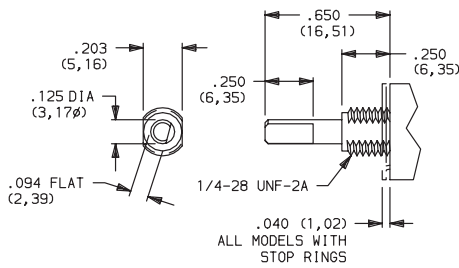
L1 .650" LONG, FLATTED
