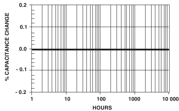
AGING RATE - NP0
