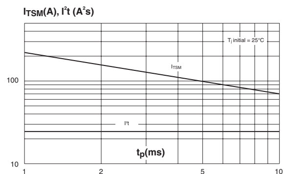
Figure 7: Non-repetitive surge peak on-state current for a sinusoidal pulse with width t_p < 10 ms, and corresponding values of I²t
