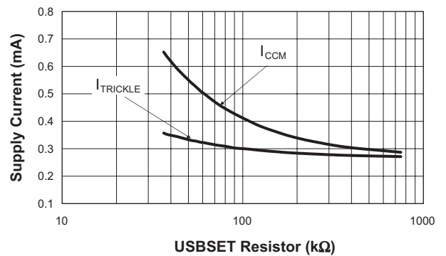
USB Mode Supply Current vs. USBSET Resistor
