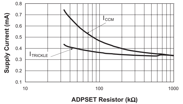
Adapter Mode Supply Current vs. ADPSET Resistor
