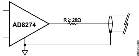
Figure 48. Driving Cabling
