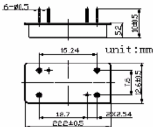
Package Outline
