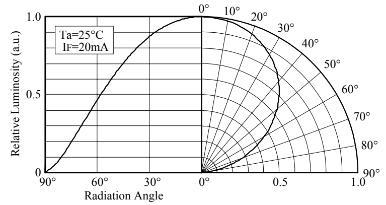
■ Directivity (NSCB455A)
