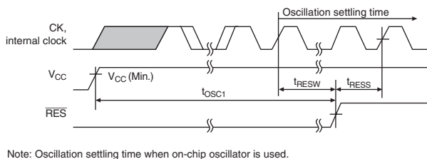
Figure 26.3 Power-On Oscillation Settling Timing
