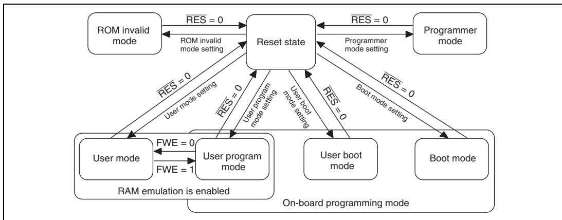
Figure 22.2 Mode Transition of Flash Memory
