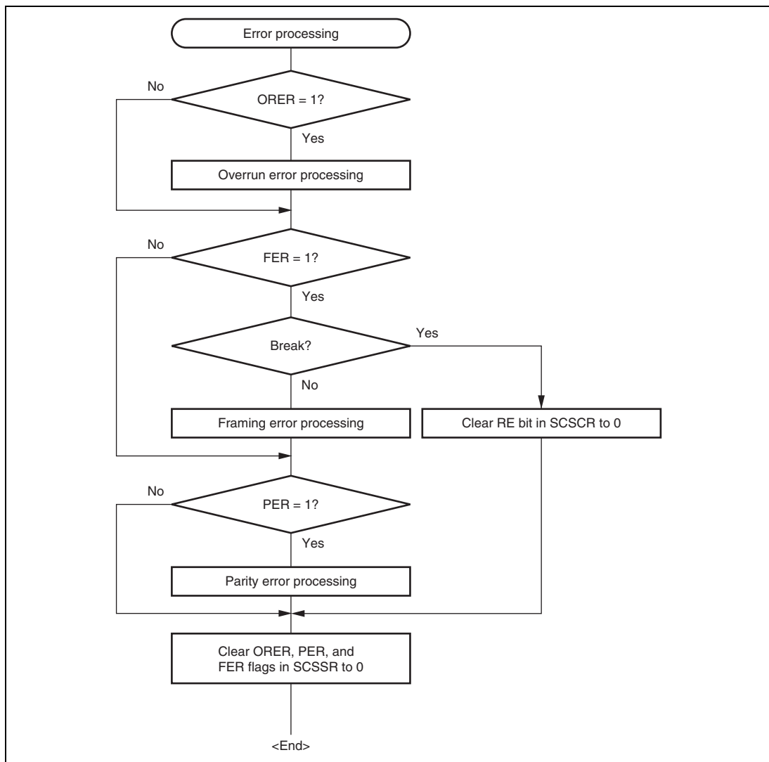
Figure 14.7 Sample Flowchart for Receiving Serial Data (2)
