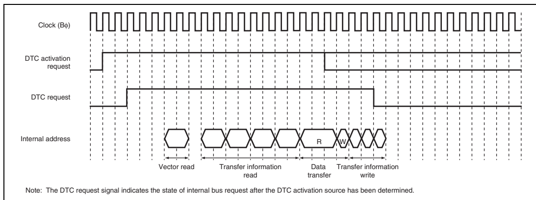
Figure 8.14 Example of DTC Operation Timing: Normal or Repeat Transfer with DTTPR = 1 (Activated by On-Chip Peripheral Module; I\phi: B\phi: P\phi = 1: 1/2: 1/2 ; Data Transferred from On-Chip Peripheral Module to On-Chip RAM; Transfer Information is Written in 3 Cycles)
