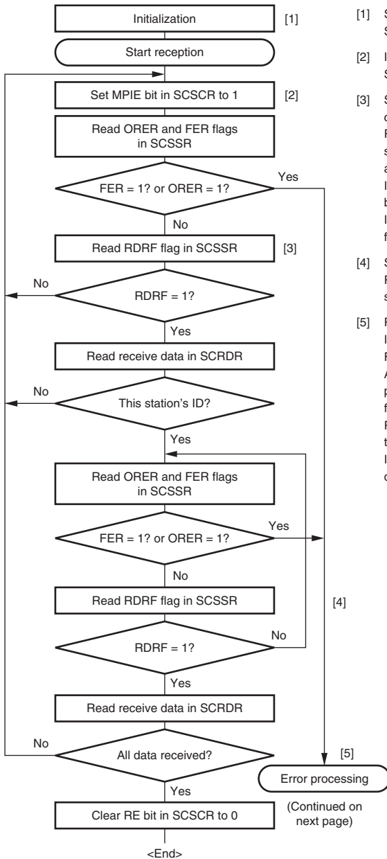
Figure 14.20 Sample Multiprocessor Serial Reception Flowchart (1)
