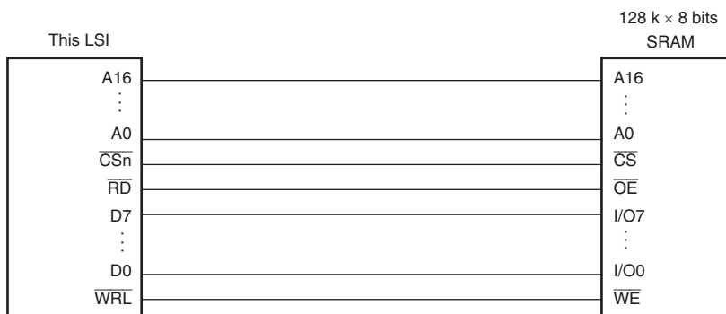
Figure 9.5 Example of 8-Bit Data-Width SRAM Connection
