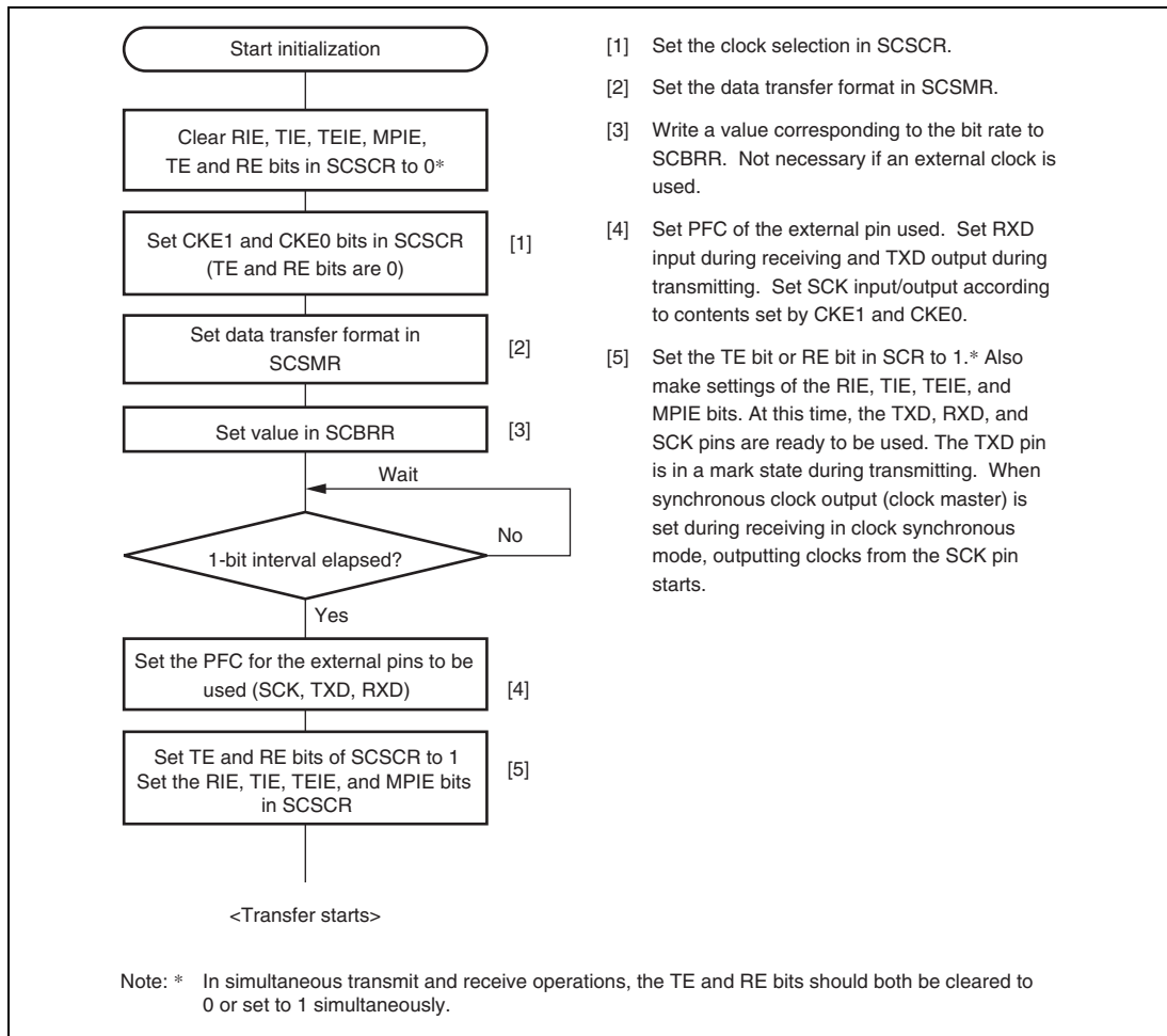
Figure 14.10 Sample Flowchart for SCI Initialization
