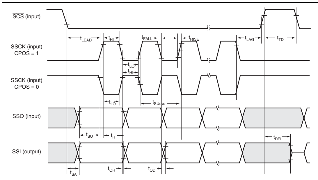
Figure 26.25 SSU Timing (Slave, CPHS = 1)
