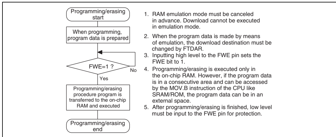
Figure 22.9 Programming/Erasing Overview Flow
