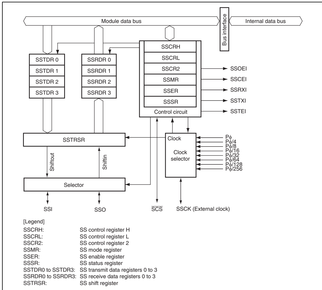
Figure 15.1 Block Diagram of SSU
