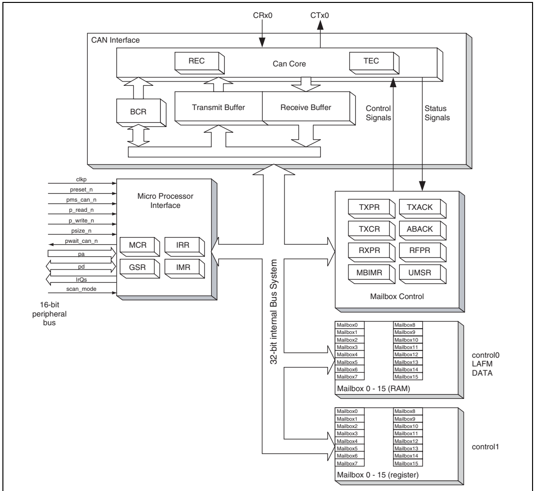
Figure 19.1 RCAN-ET Architecture
