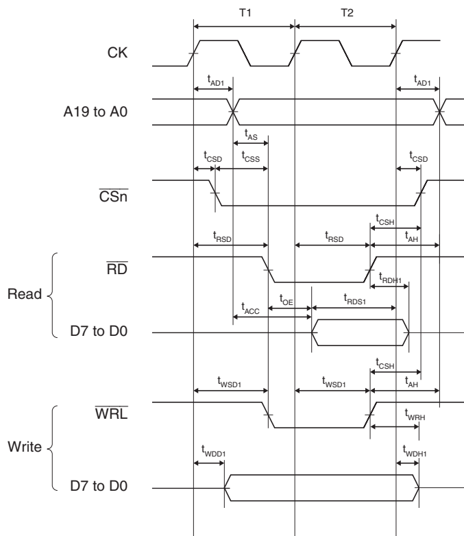
Figure 26.11 Basic Bus Timing for Normal Space (No Wait)
