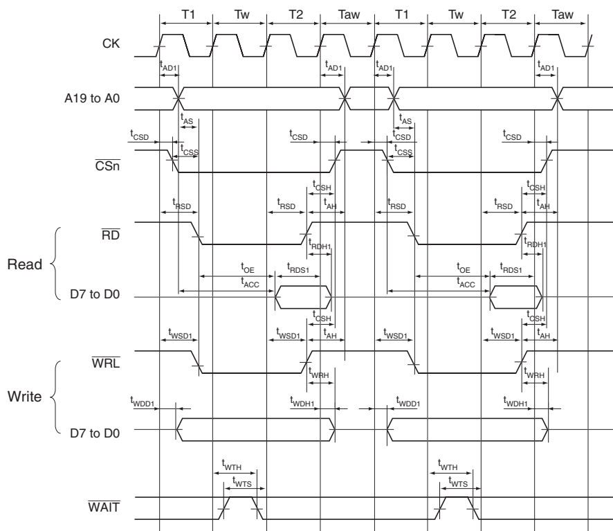
Figure 26.14 Basic Bus Timing for Normal Space (One Software Wait Cycle, External Wait Cycle Valid (WM Bit = 0), No Idle Cycle)
