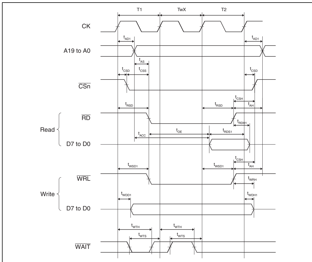
Figure 26.13 Basic Bus Timing for Normal Space (One External Wait Cycle)
