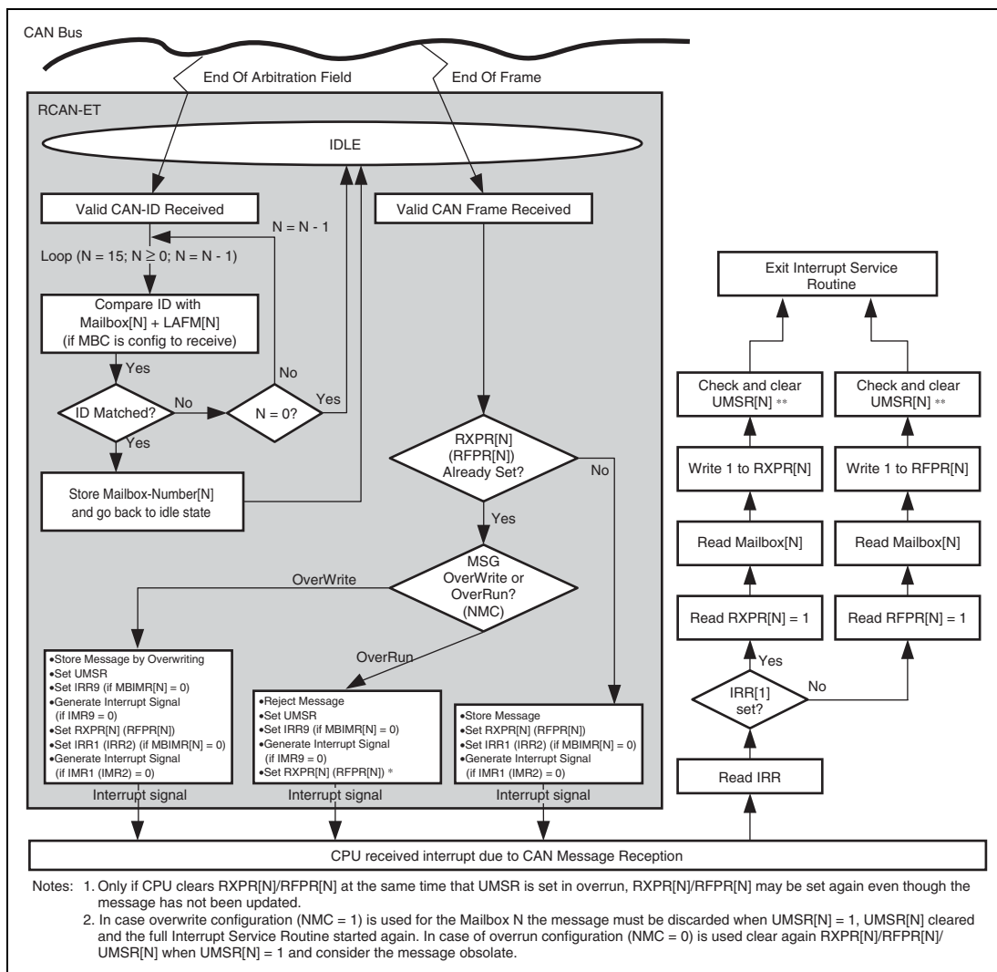
Figure 19.12 Message Receive Sequence
