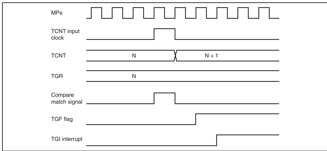
Figure 10.109 TGI Interrupt Timing (Compare Match) (Channels 0 to 4)
