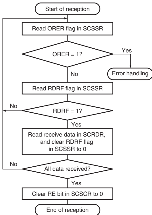
Figure 14.13 Sample Flowchart for Receiving Serial Data (1)
