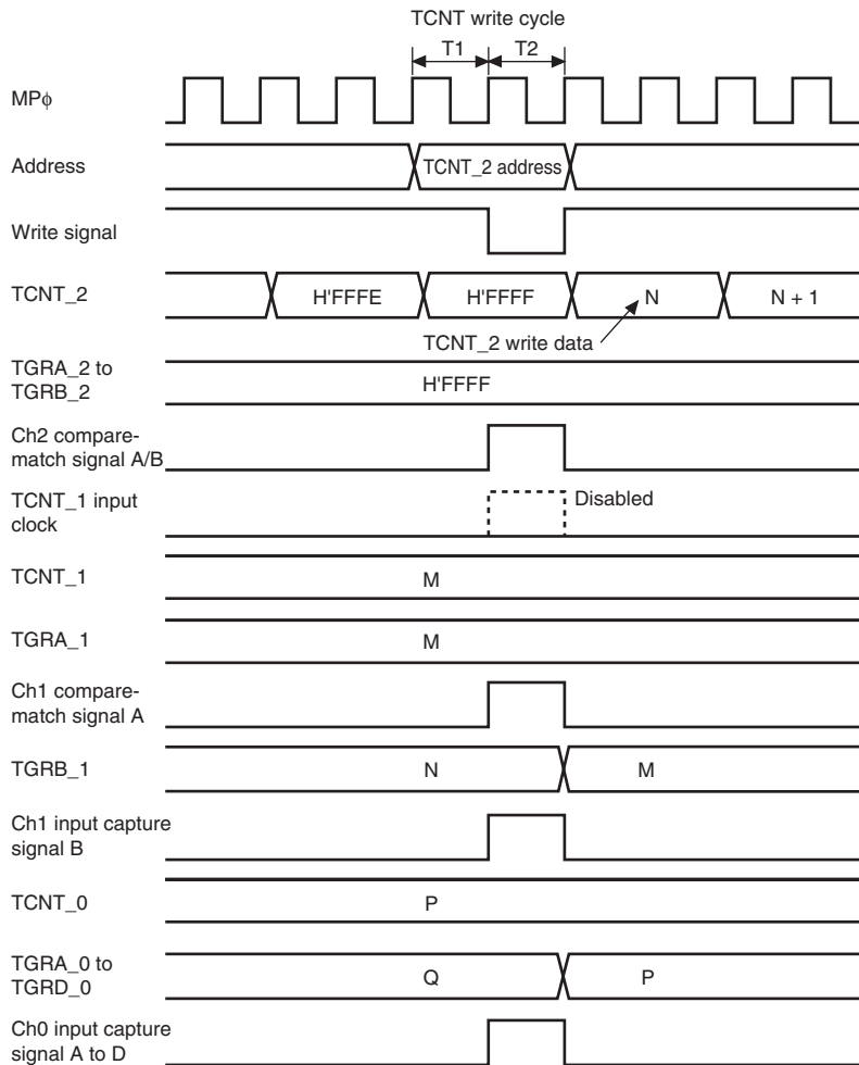
Figure 10.130 TCNT_2 Write and Overflow/Underflow Contention with Cascade Connection
