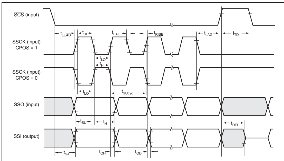
Figure 26.26 SSU Timing (Slave, CPHS = 0)
