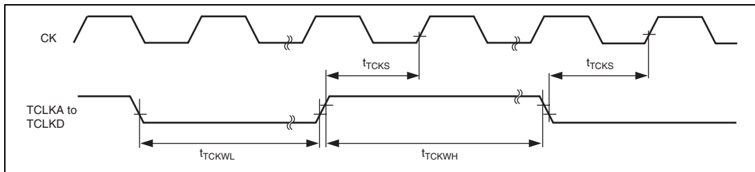
Figure 26.17 MTU2 Clock Input Timing
