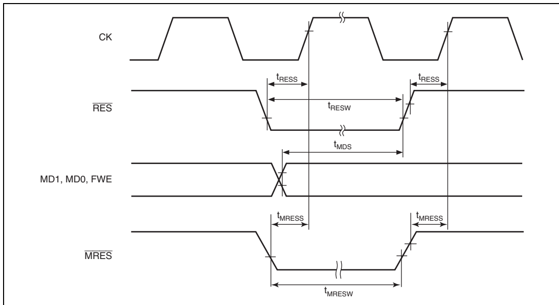
Figure 26.6 Reset Input Timing
