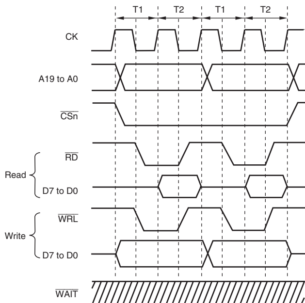
Figure 9.4 Continuous Access for Normal Space 2 Bus Width = 8 Bits, Word Access, WM Bit in CSnWCR = 1 (Access Wait = 0, Cycle Wait = 0)
