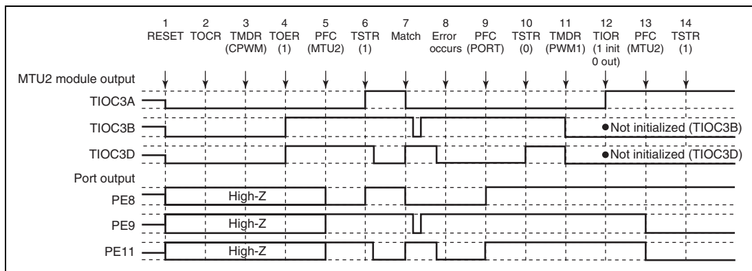
Figure 10.157 Error Occurrence in Complementary PWM Mode, Recovery in PWM Mode 1
