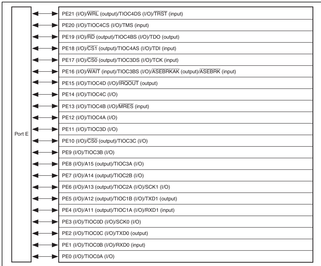
Figure 21.7 Port E (SH7137)
