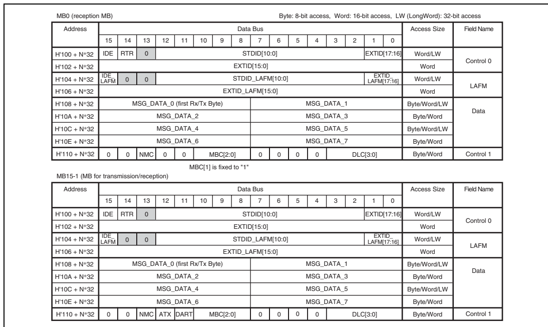
Figure 19.3 Mailbox-N Structure
