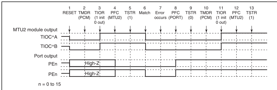
Figure 10.155 Error Occurrence in Phase Counting Mode, Recovery in Phase Counting Mode
