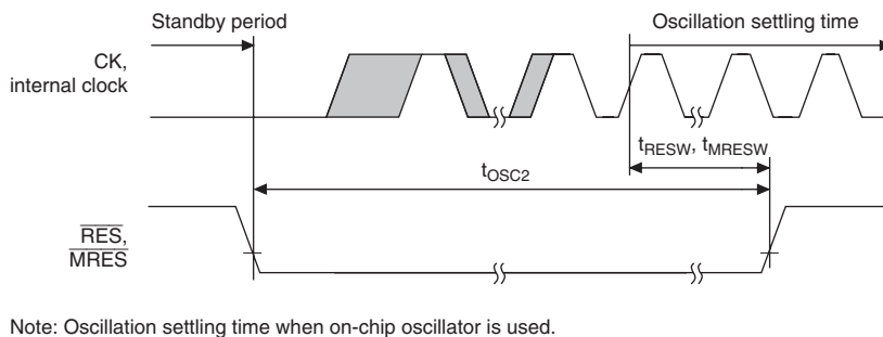
Figure 26.4 Oscillation Settling Timing on Return from Standby (Return by Reset)
