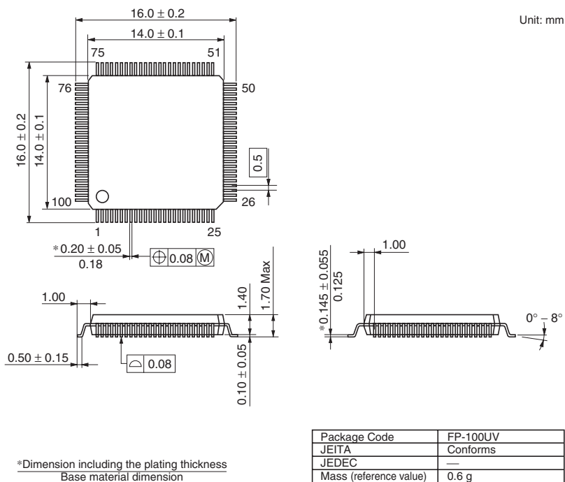
Figure D.2 FP-100UV
