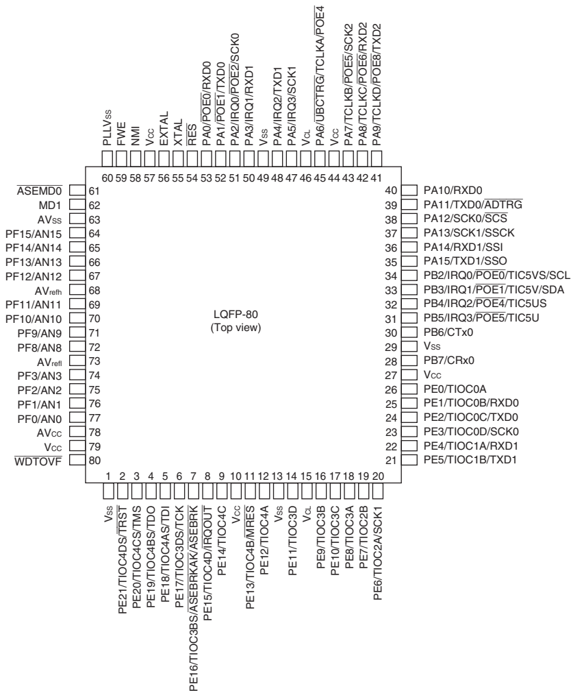
Figure 1.2 SH7136 Pin Assignments
