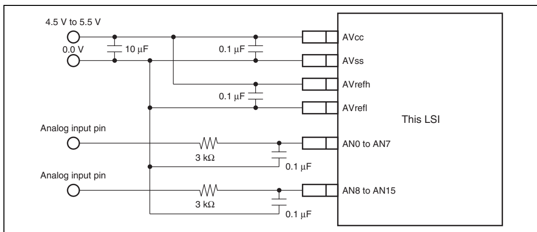
Figure 17.9 Example of Analog Input Pin Protection Circuit
