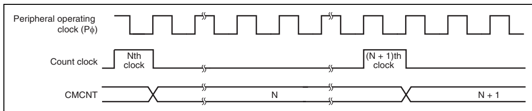
Figure 18.3 Count Timing
