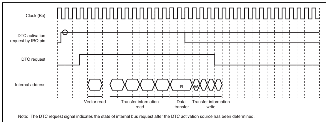
Figure 8.15 Example of DTC Operation Timing: Normal or Repeat Transfer (Activated by IRQ; I\phi: B\phi: P\phi = 1: 1/2: 1/2 ; Data Transferred from On-Chip Peripheral Module to On-Chip RAM; Transfer Information is Written in 3 Cycles)
