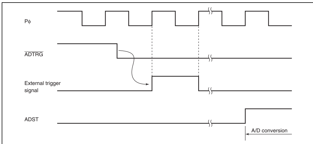
Figure 17.6 External Trigger Input Timing
