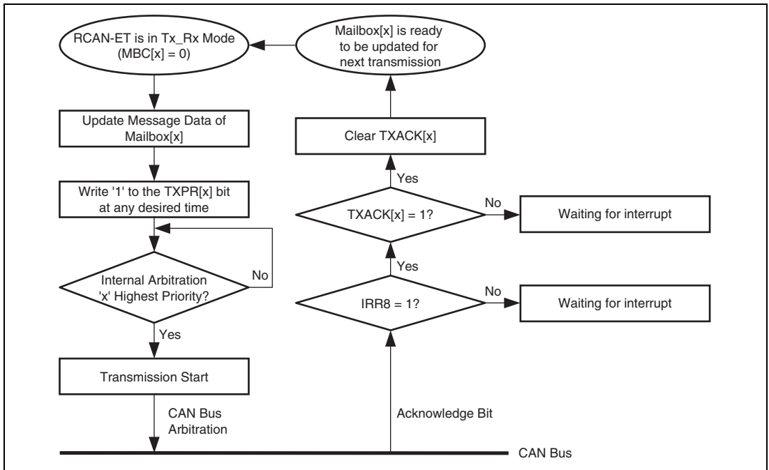
Figure 19.10 Transmission Request
