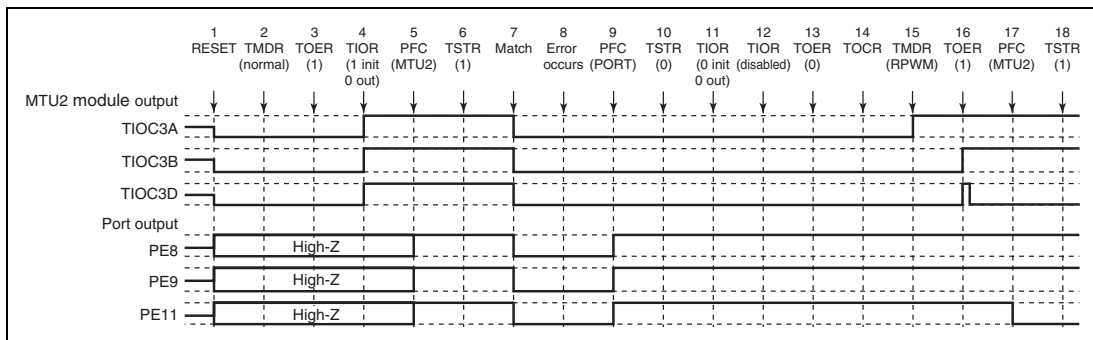
Figure 10.141 Error Occurrence in Normal Mode, Recovery in Reset-Synchronized PWM Mode
