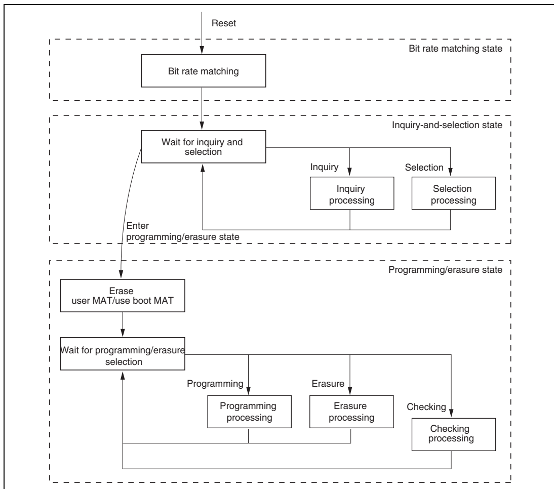
Figure 22.22 Flow of Processing by the Boot Program
