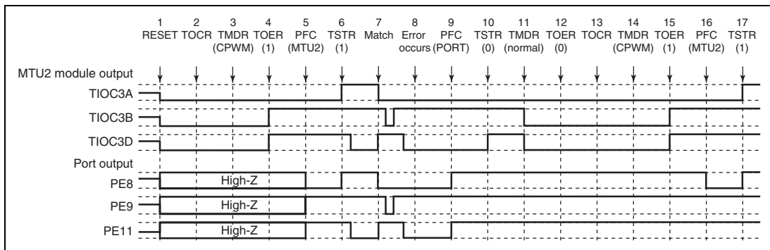
Figure 10.159 Error Occurrence in Complementary PWM Mode, Recovery in Complementary PWM Mode
