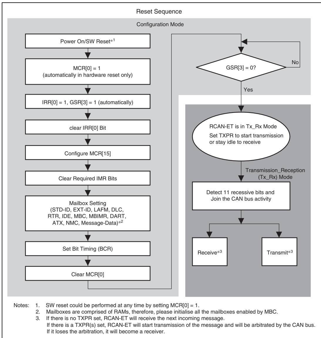
Figure 19.8 Reset Sequence
