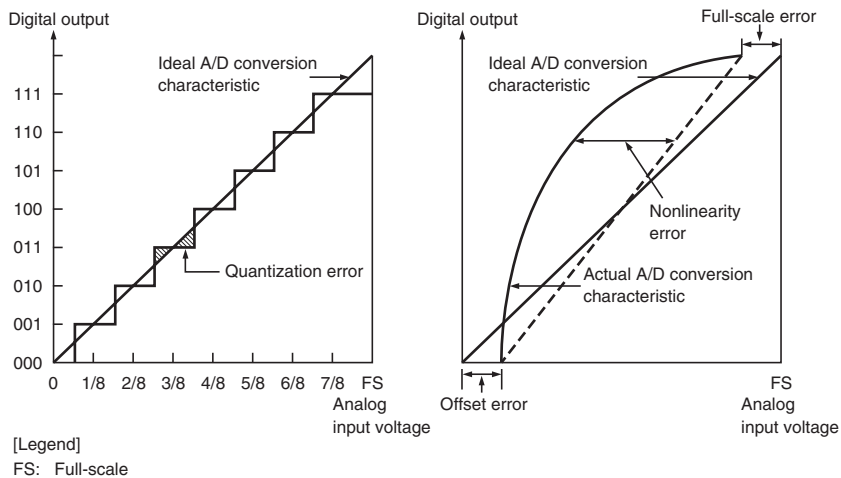
Figure 17.8 Definitions of A/D Conversion Accuracy
