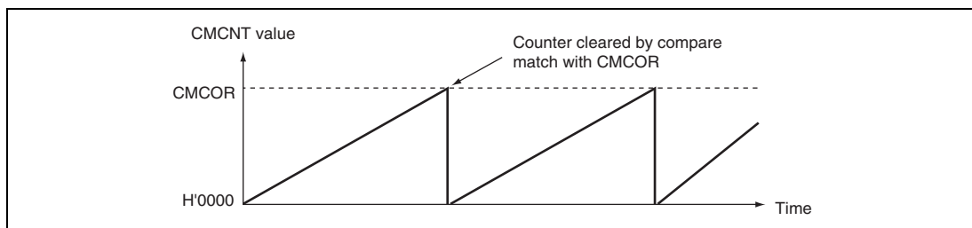
Figure 18.2 Counter Operation
