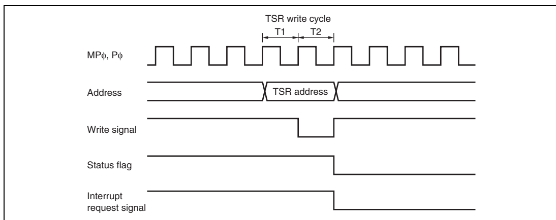
Figure 10.116 Timing for Status Flag Clearing by CPU (Channel 5)
