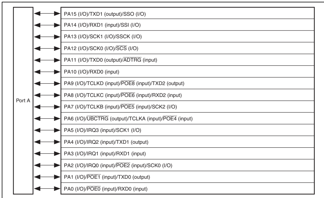
Figure 21.1 Port A (SH7136)
