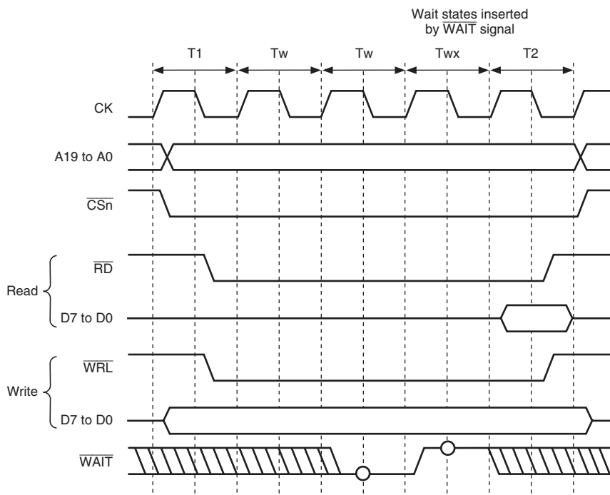
Figure 9.7 Wait State Timing for Normal Space Access (Wait State Insertion Using \overline{\text{WAIT}} Signal)
