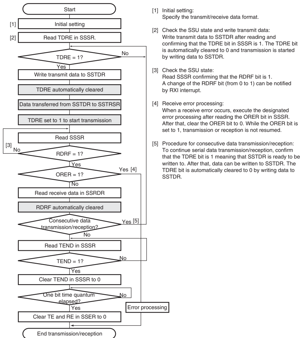
Figure 15.17 Flowchart Example of Simultaneous Transmission/Reception (Clock Synchronous Communication Mode)
