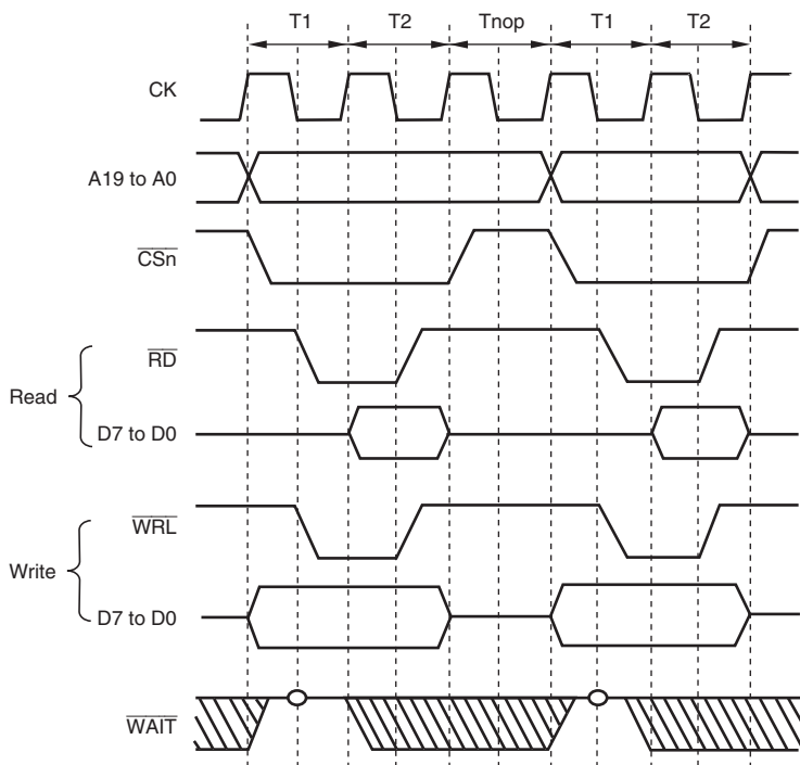
Figure 9.3 Continuous Access for Normal Space 1 Bus Width = 8 Bits, Word Access, WM Bit in CSnWCR = 0 (Access Wait = 0, Cycle Wait = 0)
