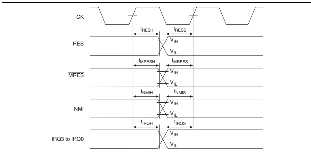
Figure 26.7 Interrupt Signal Input Timing
