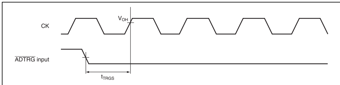
Figure 26.31 External Trigger Input Timing
