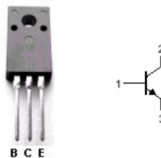
Fig.1 simplified outline (ITO-220) and symbol
