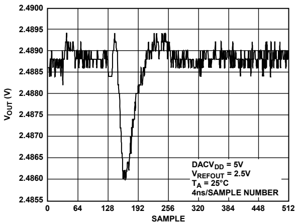
Figure 19. DAC-to-DAC Crosstalk
