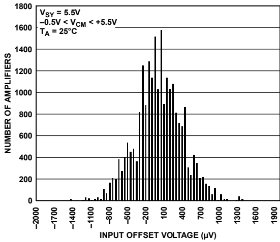
Figure 31. Amplifier Input Offset Voltage Distribution
