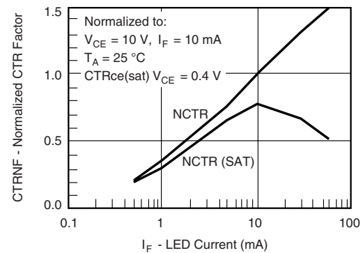
Fig. 6 - Normalized Non-Saturated and Saturated CTR vs. LED Current
