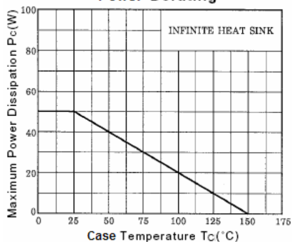
Power Derating
