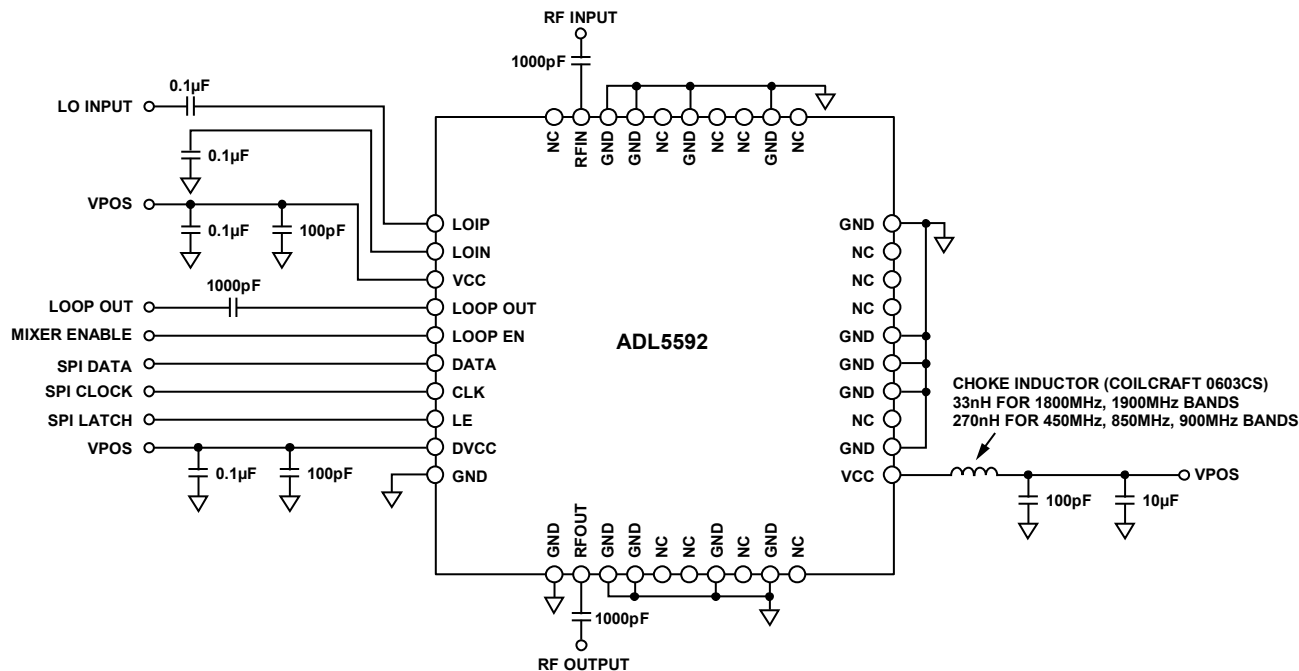
Figure 17. Basic Connections
