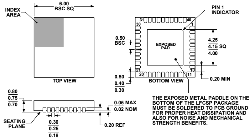
Figure 27. 40-Lead Lead Frame Chip Scale Package [LFCSP_WQ]
