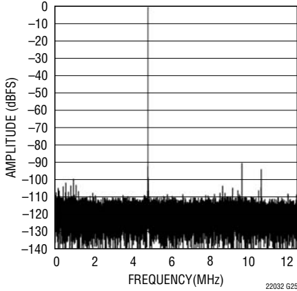
LTC2203: 32K Point FFT, f_{IN} = 70.1\text{MHz} , -1dBFS, PGA = 1
