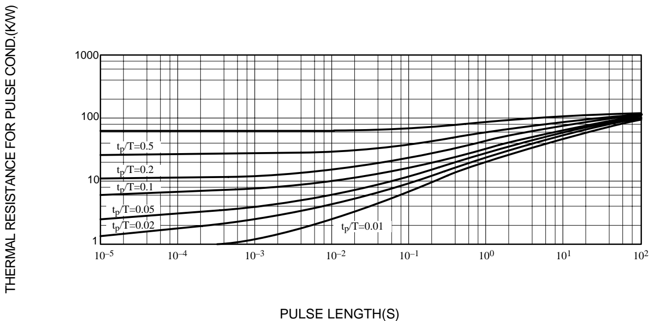
FIG.3 – THERMAL RESPONSE
