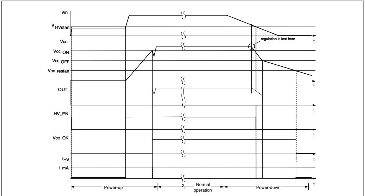
Figure 36. Timing diagram: normal power-up and power-down sequences
