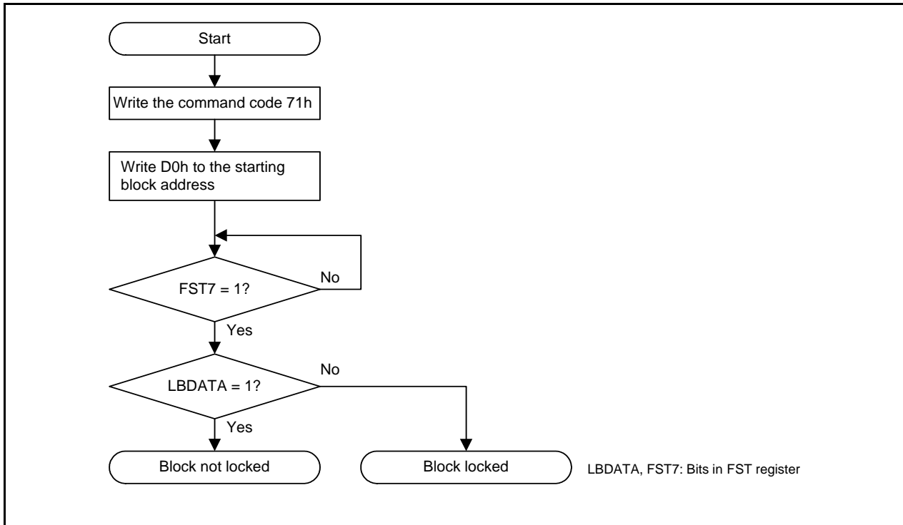
Figure 31.13 Read Lock Bit Status Flowchart
