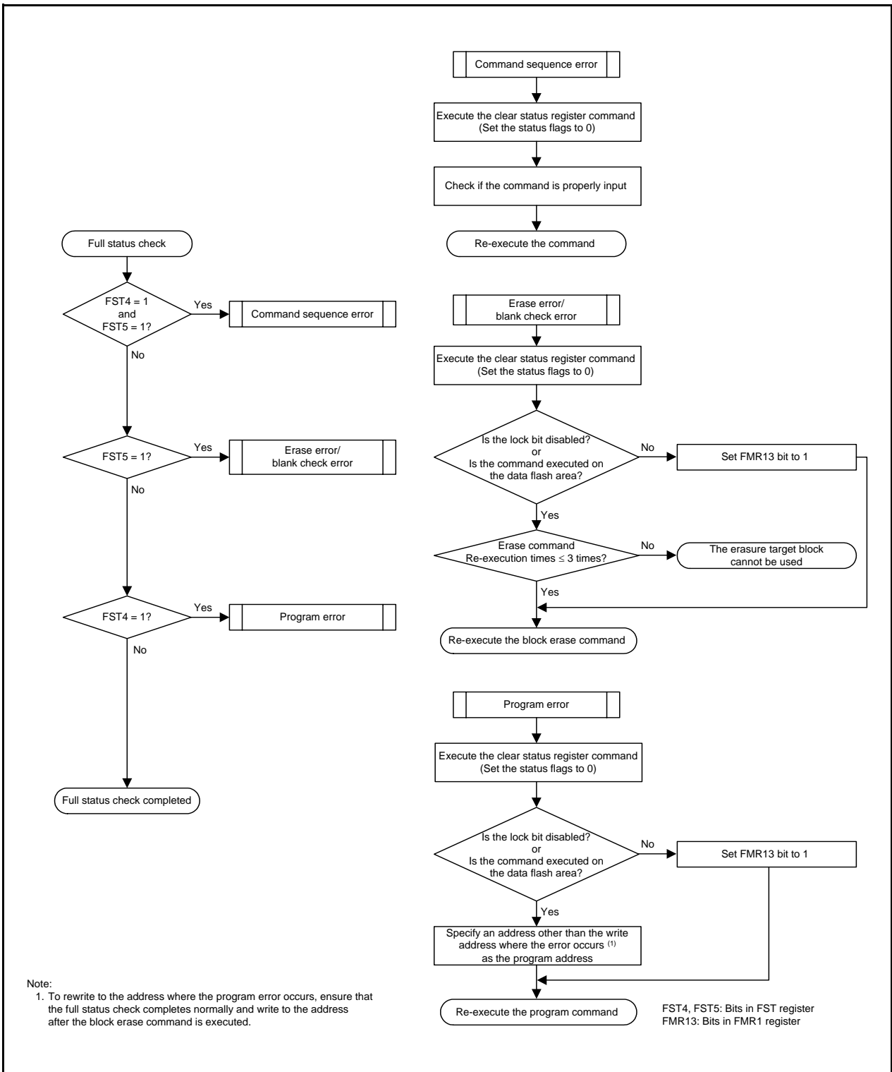
Figure 31.15 Full Status Check and Handling Procedure for Individual Errors
