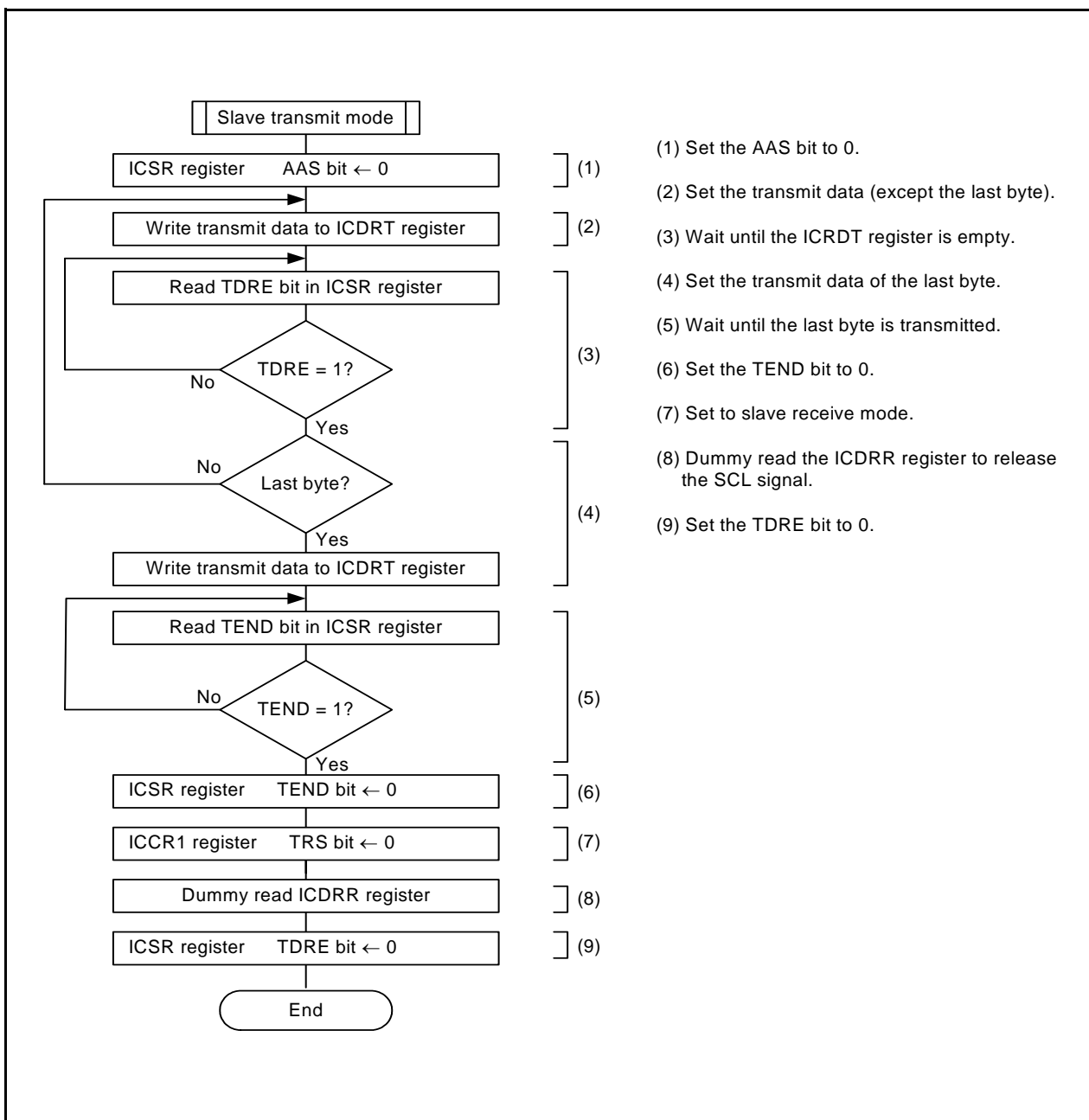
Figure 25.17 Register Setting Example in Slave Transmit Mode (I 2 C bus Interface Mode)
