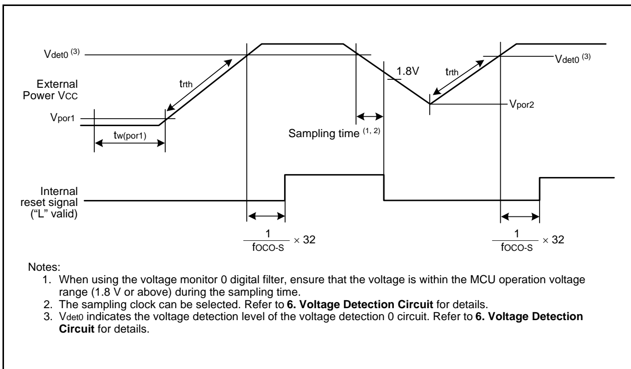
Figure 33.3 Power-on Reset Circuit Electrical Characteristics
