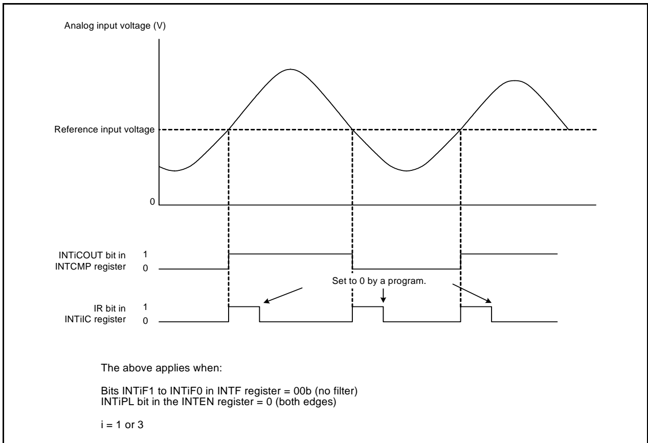
Figure 30.2 Operating Example of Comparator Bi (i = 1 or 3)
