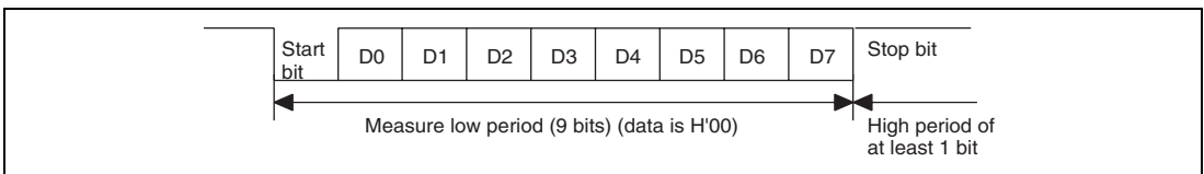
Figure 21.7 Automatic Adjustment Operation of SCIF Bit Rate
