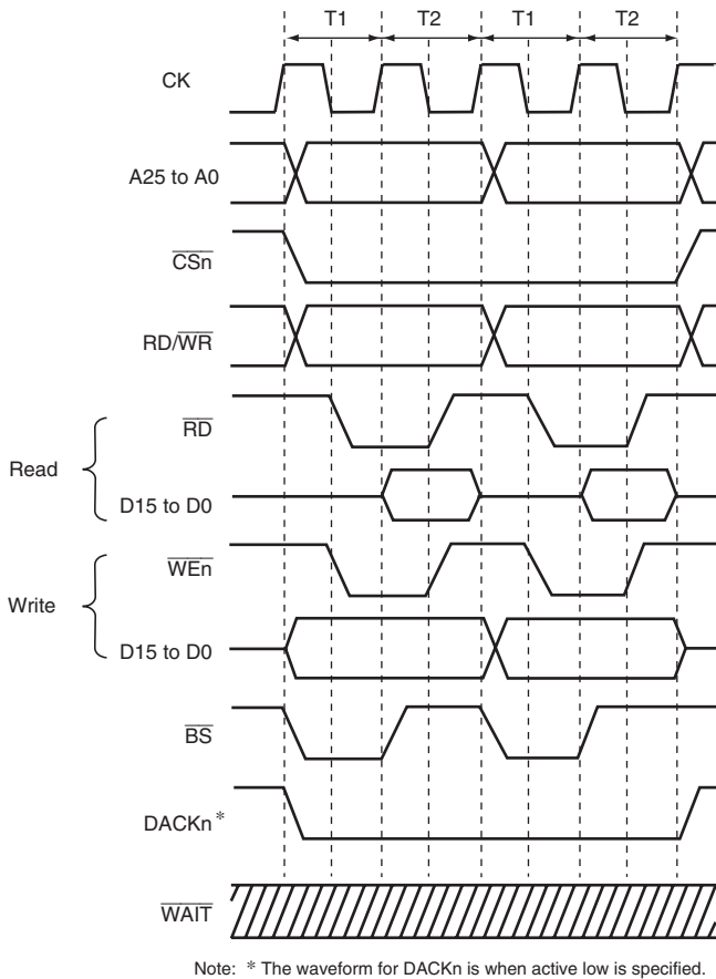
Figure 8.4 Continuous Access for Normal Space 2 Bus Width = 16 Bits, Longword Access, CSnWCR.WM Bit = 1 (Access Wait = 0, Cycle Wait = 0)
