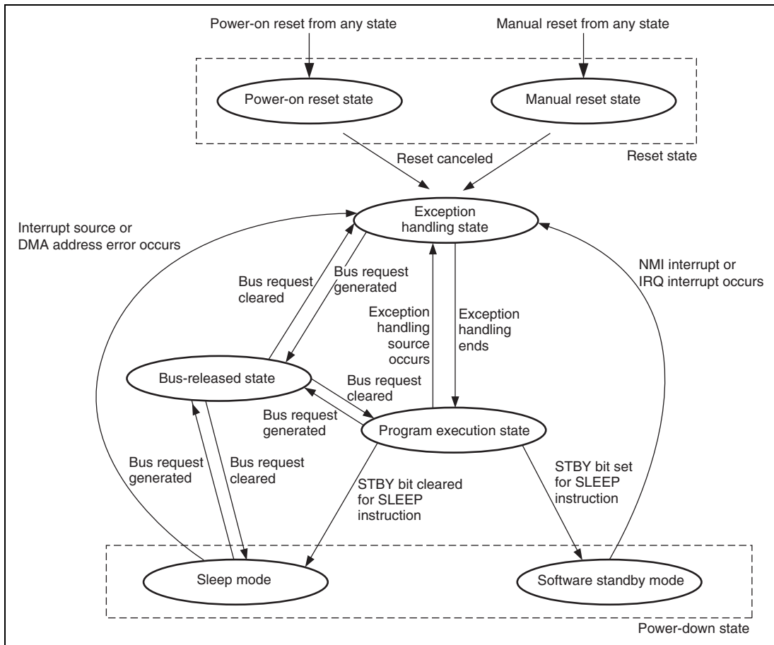
Figure 2.6 Transitions between Processing States
