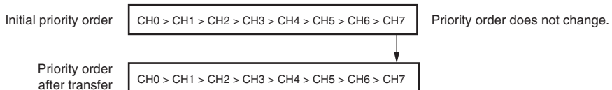
Figure 9.3 Round-Robin Mode
