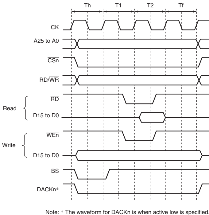
Figure 8.9 \overline{\text{CSn}} Assert Period Expansion
