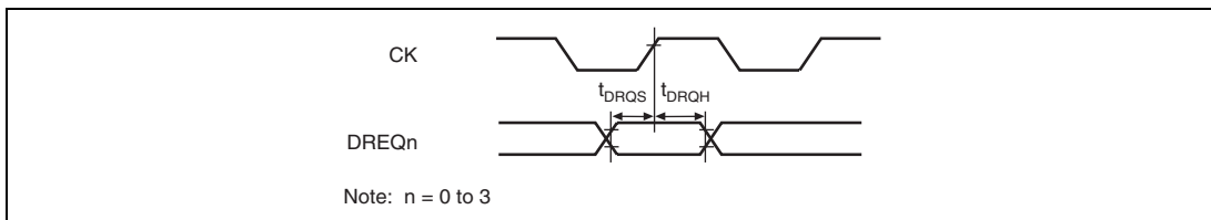
Figure 27.40 DREQ Input Timing
