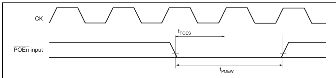
Figure 27.44 POE2 Input/Output Timing
