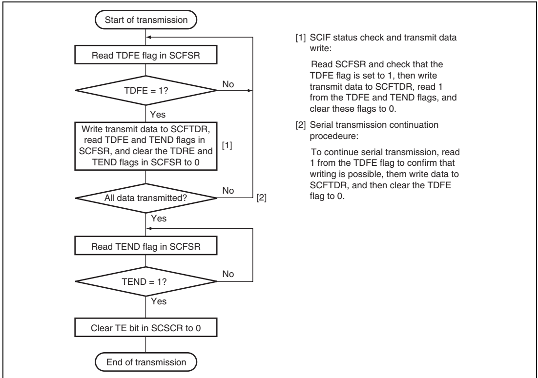
Figure 15.11 Sample Flowchart for Transmitting Serial Data
