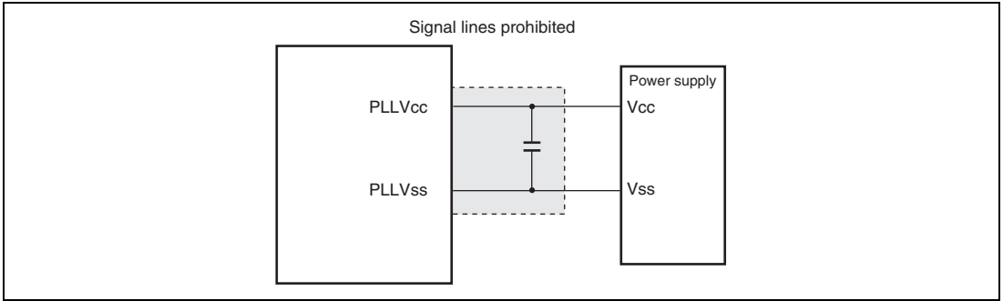
Figure 4.3 Note on Using a PLL Oscillation Circuit
