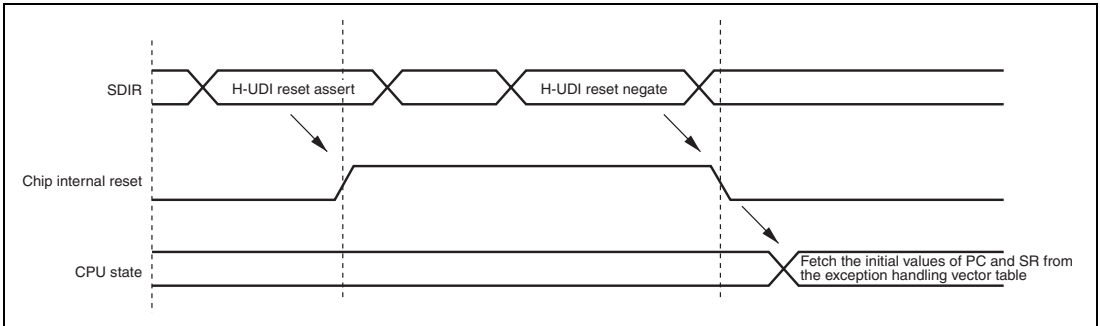
Figure 24.4 H-UDI Reset
