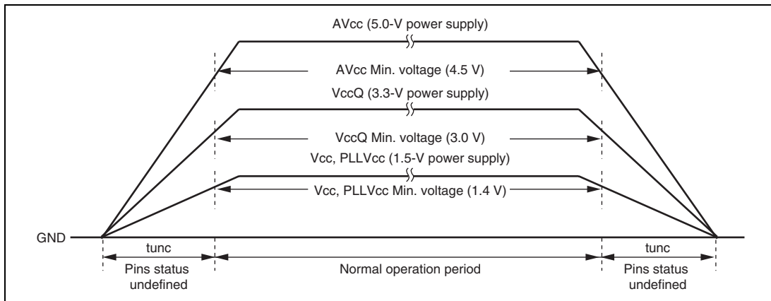
Figure 27.1 Power-on/Power-off Sequence
