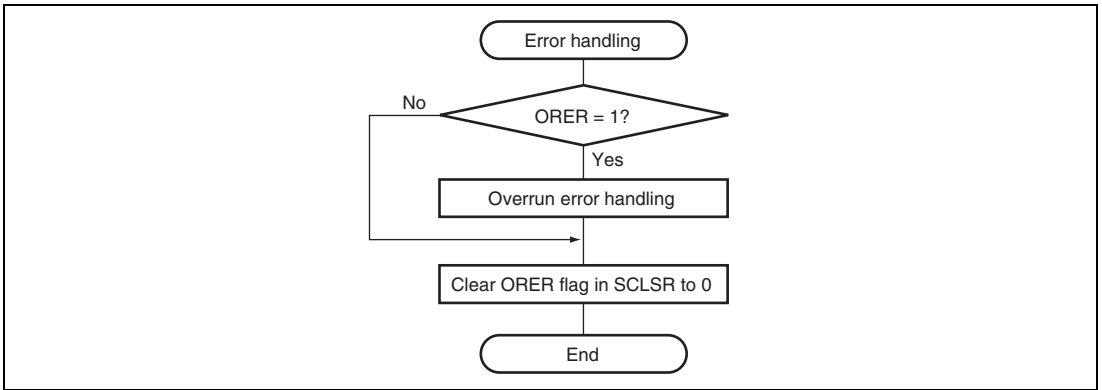
Figure 15.14 Sample Flowchart for Receiving Serial Data (2)
