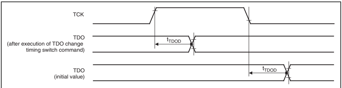
Figure 24.3 H-UDI Data Transfer Timing
