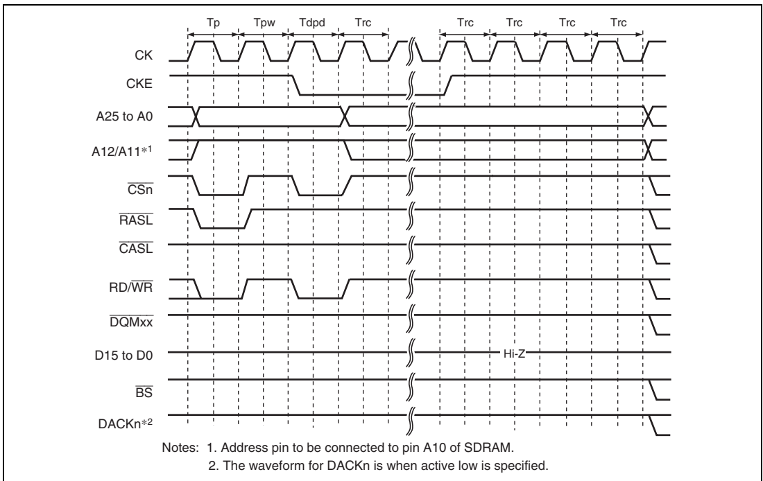
Figure 8.31 Deep Power-Down Mode Transition Timing
