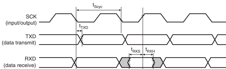
Figure 27.47 SCIF Input/Output Timing in Clocked Synchronous Mode
