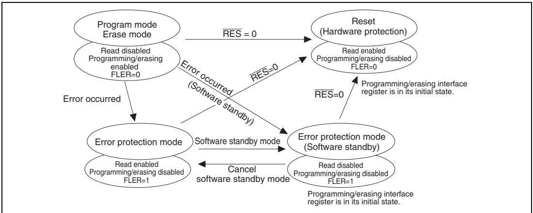
Figure 21.16 Transitions to and from Error Protection State
