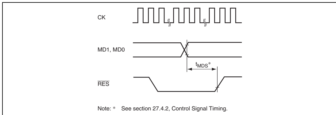
Figure 3.2 Reset Input Timing when Changing Operating Mode
