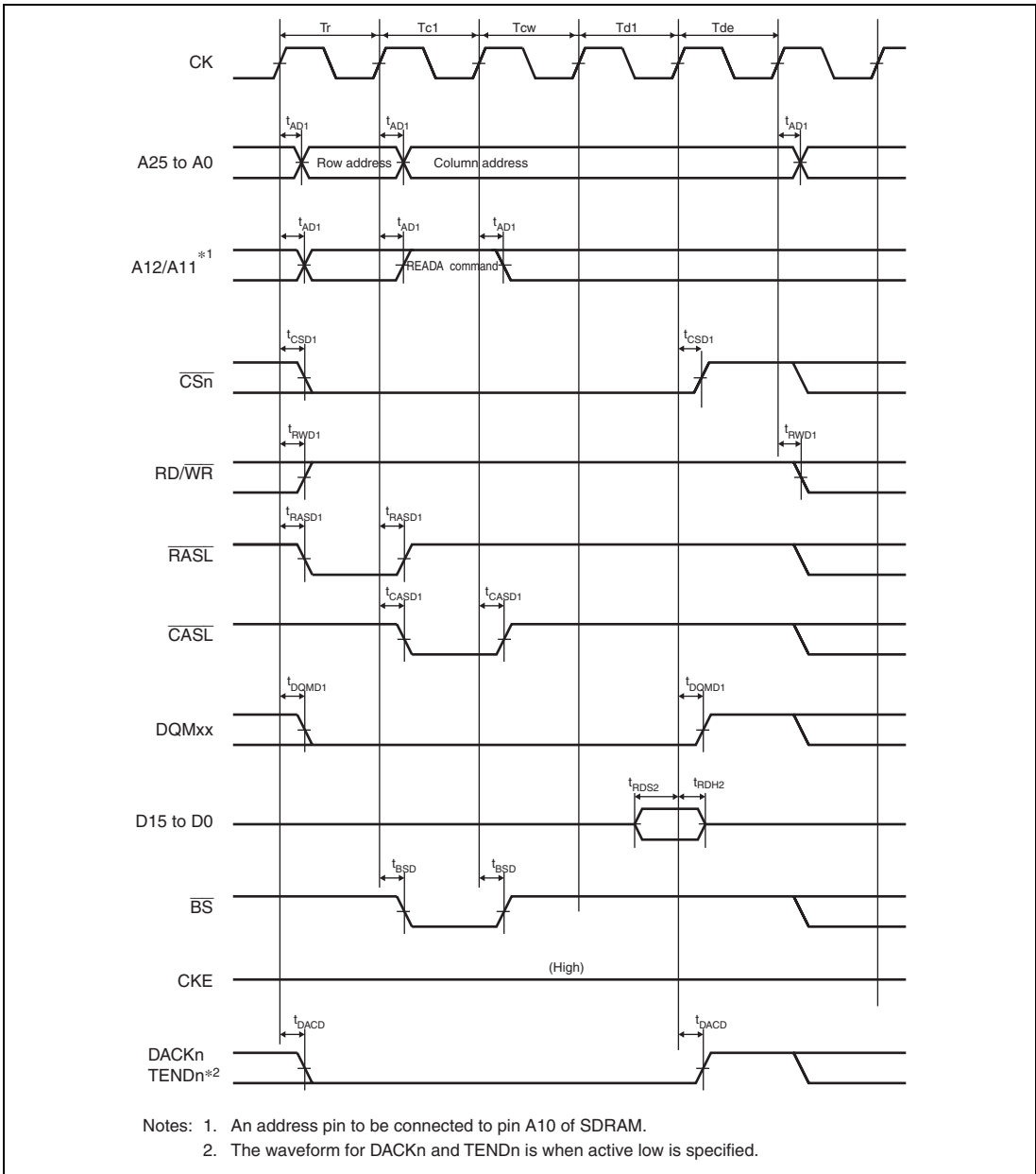
Figure 27.20 Synchronous DRAM Single Read Bus Cycle (Auto Precharge, CAS Latency 2, WTRCD = 0 Cycle, WTRP = 0 Cycle)
