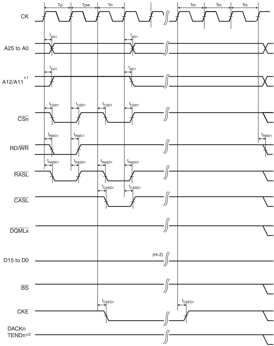
Figure 27.35 Synchronous DRAM Self-Refreshing Timing (WTRP = 1 Cycle)
