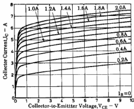
Fig.3 Static Characteristic
