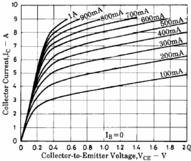
Fig.3 Static Characteristic
