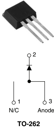
TO-262
