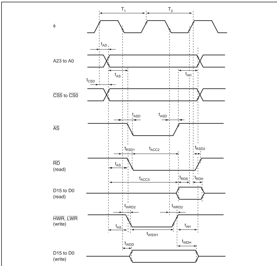
Figure 22.7 Basic Bus Timing (Two-State Access)
