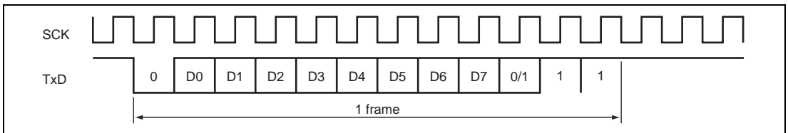
Figure 12.7 Relationship between Output Clock and Transfer Data Phase (Asynchronous Mode)
