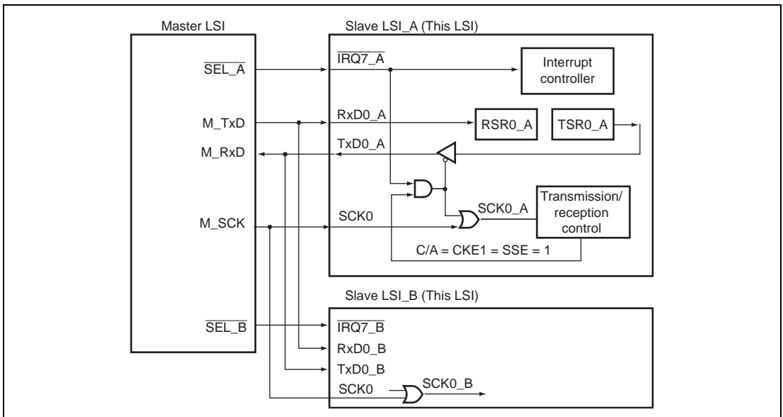
Figure 12.36 Example of Communication Using the SCI Select Function
