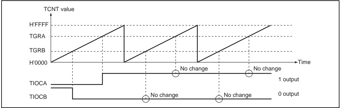
Figure 9.10 Example of 0 Output/1 Output Operation
