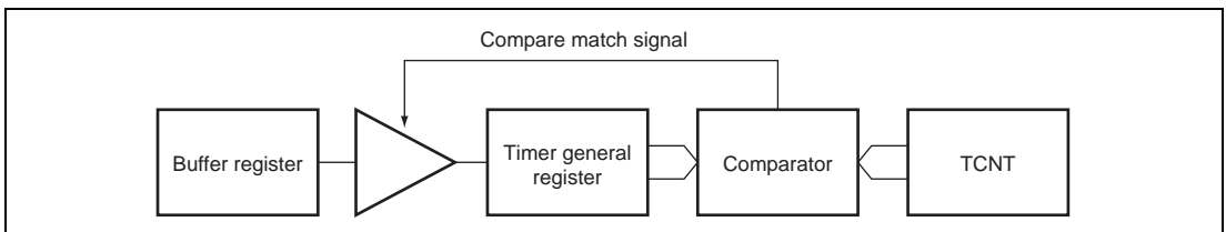
Figure 9.16 Compare Match Buffer Operation
