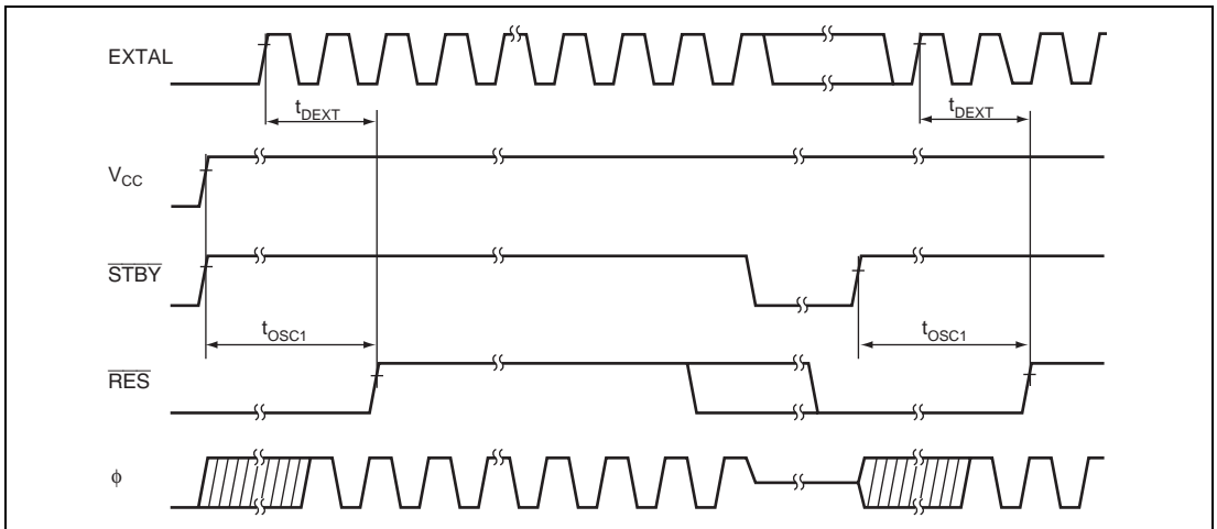
Figure 22.4 Oscillation Stabilization Timing
