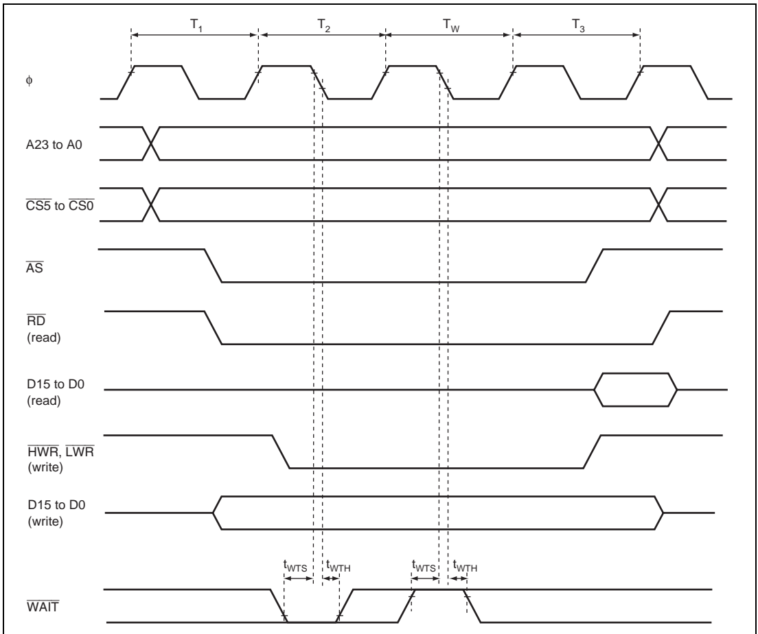
Figure 22.9 Basic Bus Timing (Three-State Access with One Wait State)
