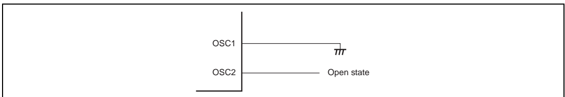
Figure 19.8 Pin Handling when Subclock Not Required
