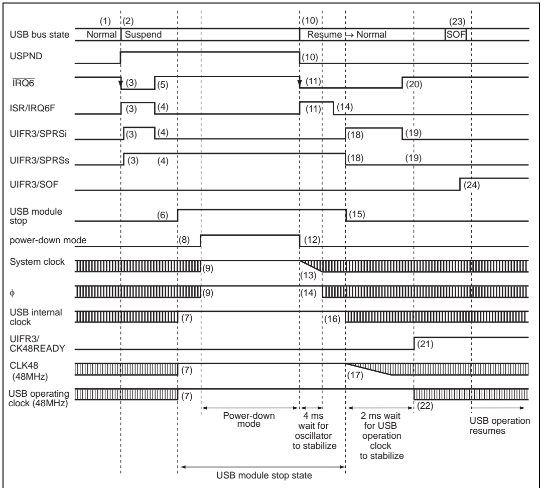
Figure 14.29 Timing Chart
