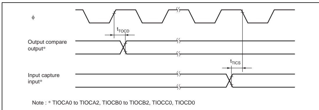
Figure 22.13 TPU Input/Output Timing
