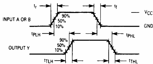
Figure 1. Switching Waveforms
