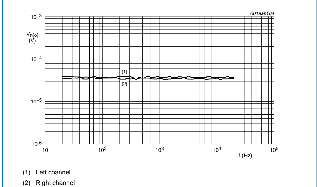
Fig 5. RMS output noise voltage as a function of frequency
