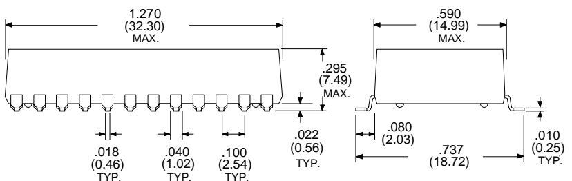
Gull wing SMD Package Add suffix "G" to P/N. Example: SP24A-105G
