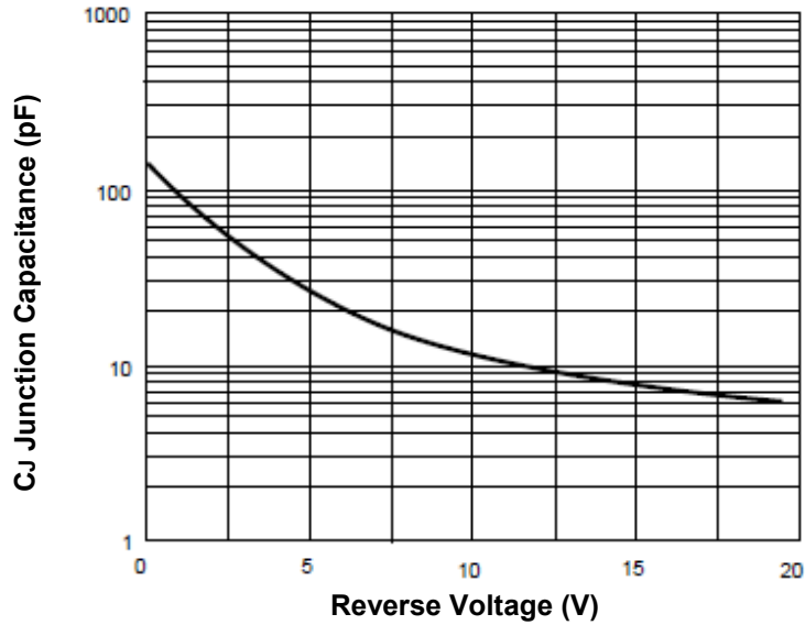
Fig.5-Typical junction capacitance
