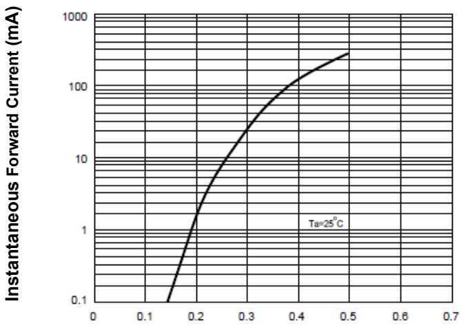
Instantaneous Forward Voltage (V) Fig.3- Typical Forward Characteristics
