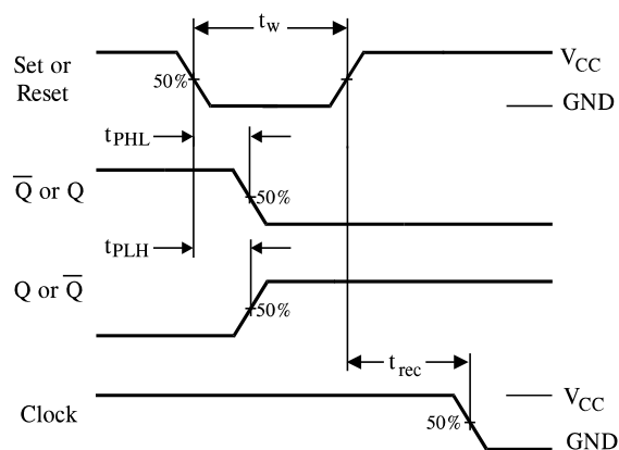
Figure 2. Switching Waveform
