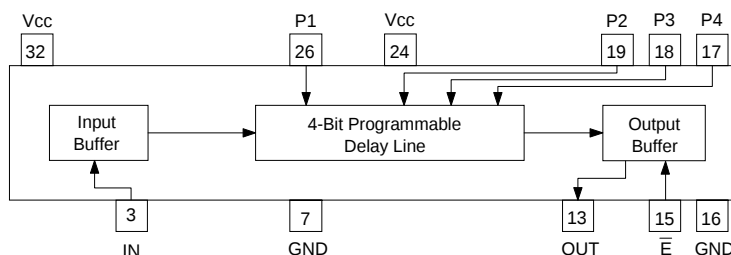
FAST / TTL 4-Bit Schematic
