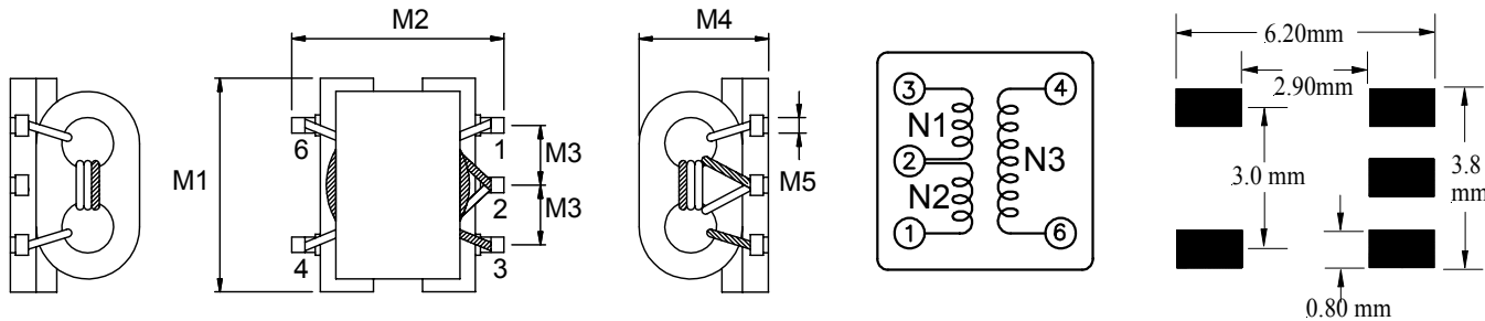
Mechanical dimension
