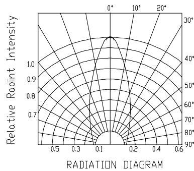
Radiation Diagram Ta=25°
