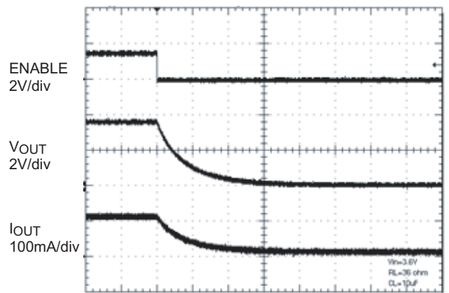
Turn-Off Timing
