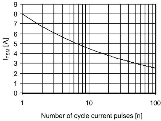
Maximum surge current d.s. cooled
