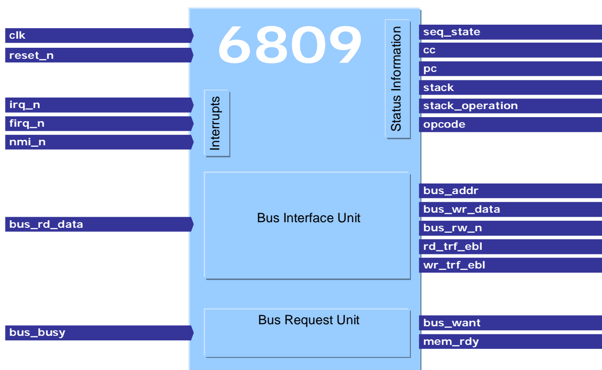
Figure 1: Logic Symbol
