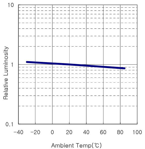
(4) Ambient Temperature vs Relative Luminosity
