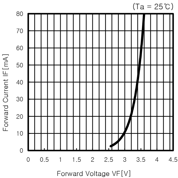
(3) Forward Current vs Forward Voltage (I F -V F )
