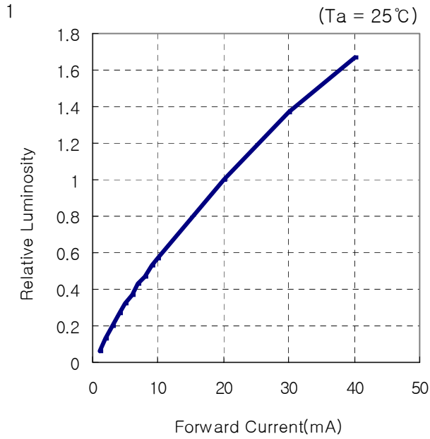
(1) Relative Luminous Intensity vs Forward Current (I F -I v )
