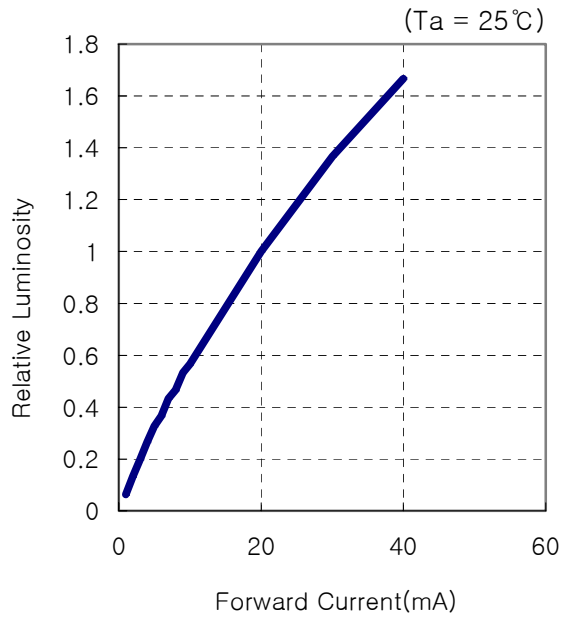
(1) Relative Luminous Intensity vs Forward Current ( I_f - I_v )
