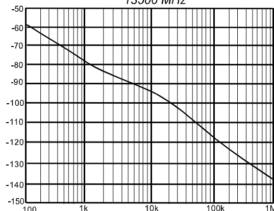
Phase Noise (dBc/Hz) 13500 MHz
