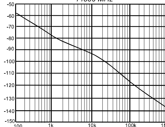
Phase Noise (dBc/Hz) 14500 MHz
