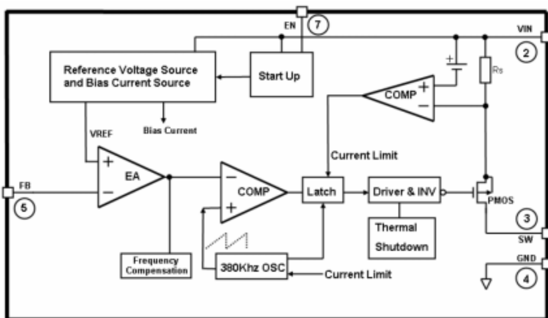
Figure 3: Function Block
