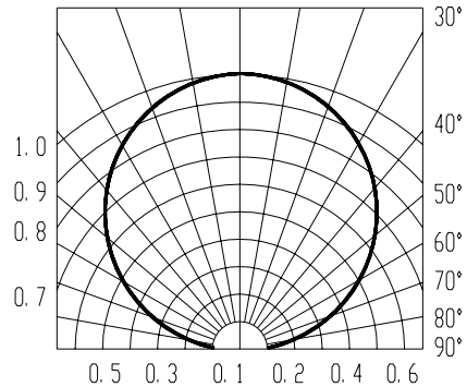
Radiation Diagram T_a=25^\circ
