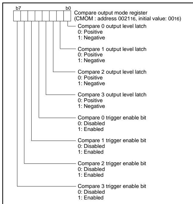
Fig. 29 Structure of compare output mode register
