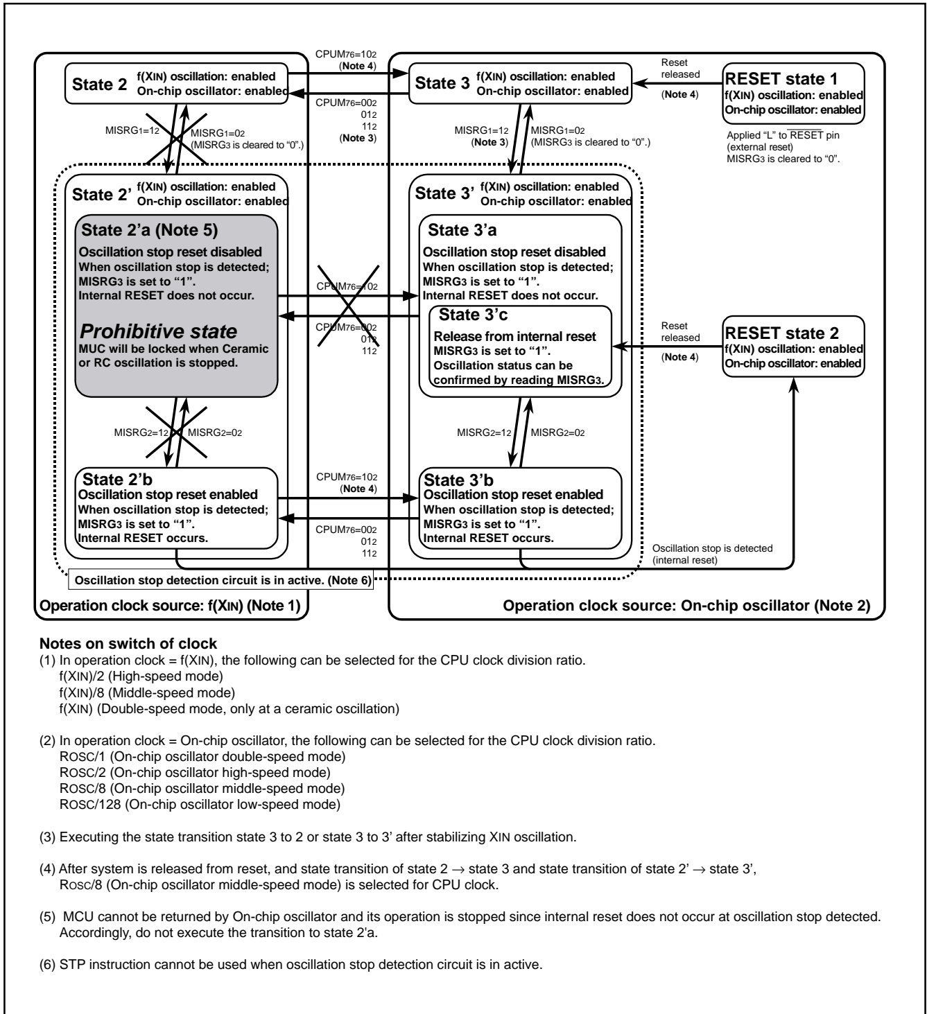
Fig. 77 State transition 2
