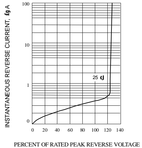
Fig. 4-REVERSE CHARACTERISTICS
