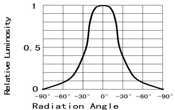
Fig 6. Relative Luminous Intensity vs. Radiation Angle
