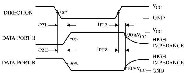
Figure 6. Switching Waveforms
