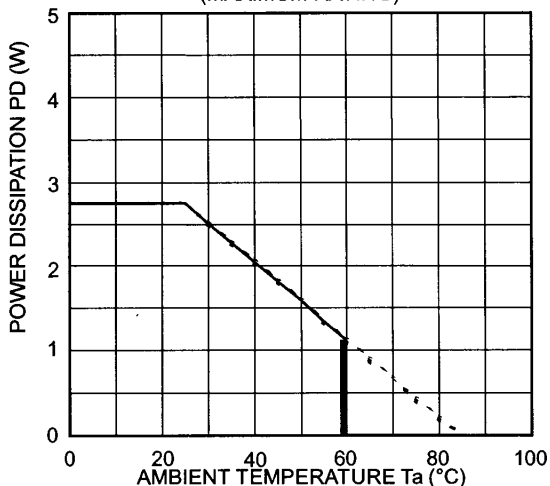
POWER DISSIPATION - AMBIENT TEMPERATURE (MAXIMUM RATING)
