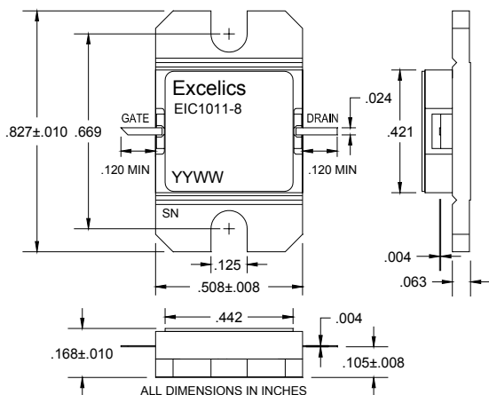
EIC1011-8 (Hermetic)
