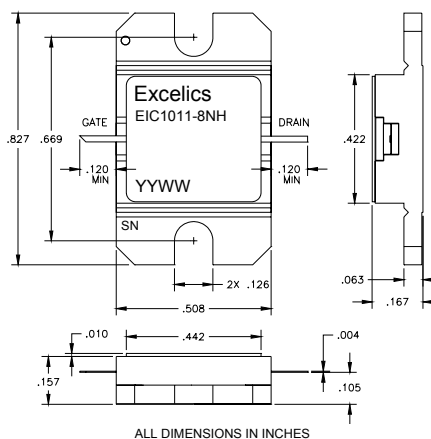
EIC1011-8NH (Non-Hermetic)
